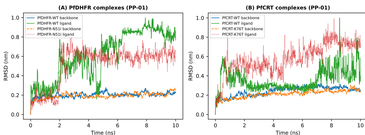
Figure 3.3.2: Pose retention and thermal equilibration for the PP-01 systems of the resistance-scoring study over 10 ns (canonical R1 trajectories). Explicit-solvent backbone (solid) and ligand-after-backbone-fit (dashed/dotted) RMSD time-series computed with gmx rms after PBC-whole reconstruction (fit group: backbone); axes in nm. Panel (A), Pf DHFR: backbone 0.203(24) nm (WT) and 0.193(29) nm (N51I); ligand 0.613(240) nm and 0.519(190) nm. Panel (B), Pf CRT: backbone 0.241(48) nm (WT) and 0.211(39) nm (K76T); ligand 0.357(113) nm and 0.581(155) nm. All four trajectories pass the geometric quality-control gate (mean minimum heavy-atom distance 2.7 to 3.2 Å, bound fraction 1.000); ligand RMSD reflects in-pocket mobility, not dissociation. No ligand dissociation was observed at single-replicate scope.
