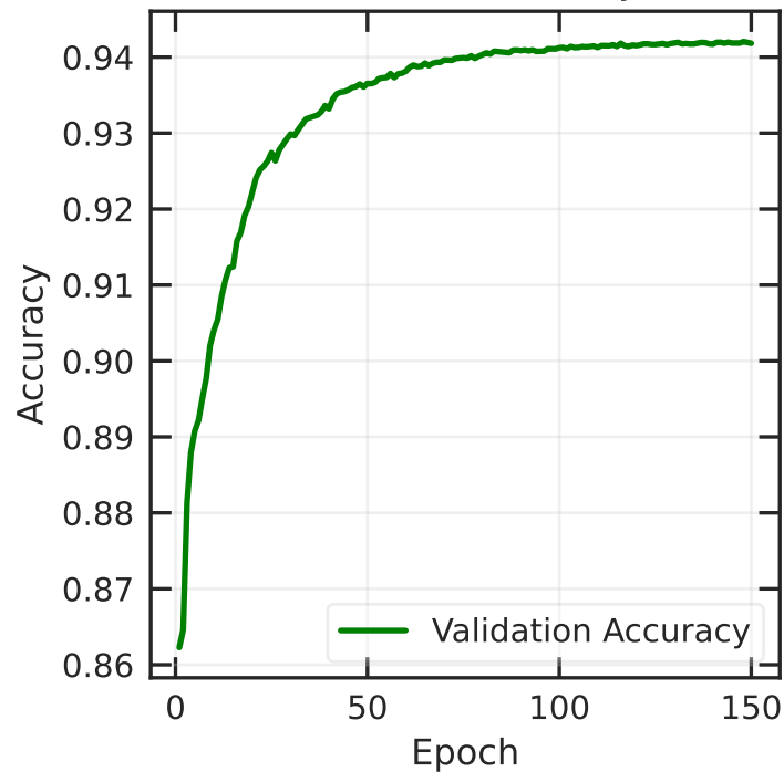
Validation Accuracy
