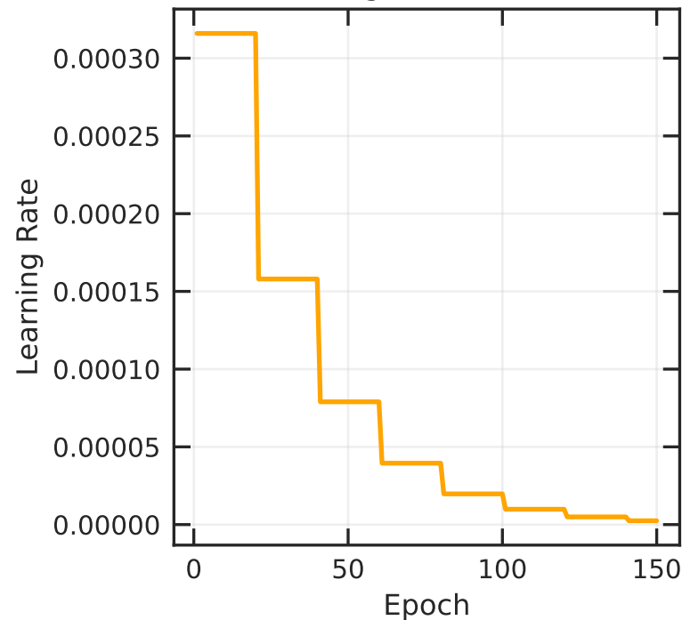
Learning Rate Schedule
