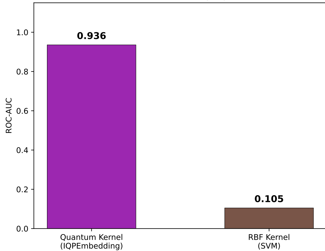
Quantum Kernel Advantage (p=0.0003)
