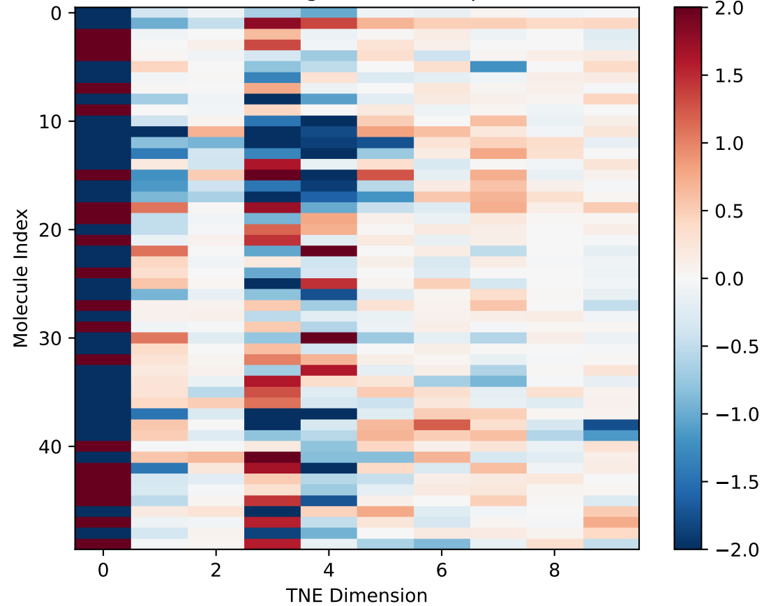
TNE Embeddings (15.6× compression)
