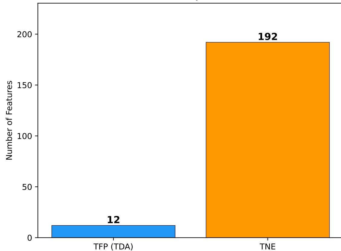
Dimensionality Reduction
