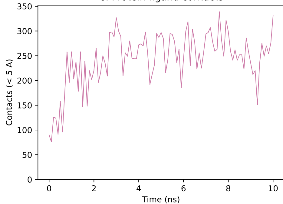
C. Protein-ligand contacts
