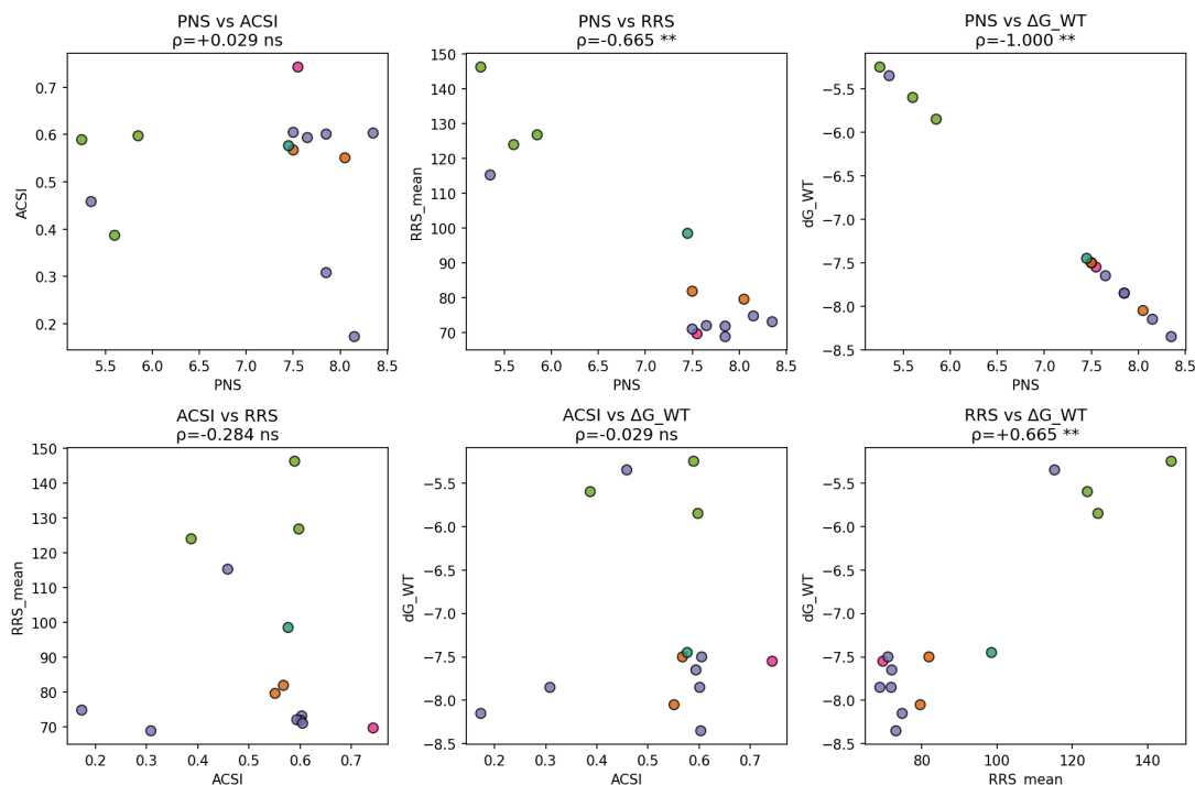
Figure 5: Cross-metric correlation matrix for the 14 candidates with complete data. Spearman \rho values between PNS, ACSI, RRS, and \Delta G_{WT} . Asterisks indicate Bonferroni-corrected significance (** p < 0.01 ). PNS vs. \Delta G_{WT} shows \rho = -1.000 due to mechanical linkage (see text).
