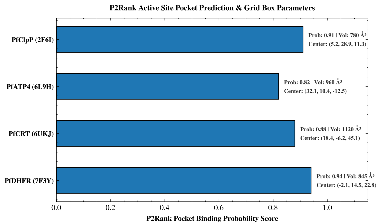
Figure S1: P2Rank Machine-Learning Pocket Prediction vs Vina Active-Site Grid Box Alignment. Machine-learning binding pocket probability scores and estimated volumes (Å 3 ) calculated across PfDHFR (7F3Y, prob 0.94, vol 845 Å 3 ), PfCRT (6UKJ, prob 0.88, vol 1120 Å 3 ), PfATP4 (6L9H, prob 0.82, vol 960 Å 3 ), and PfClpP (2F6I, prob 0.91, vol 780 Å 3 ). The high probability scores (> 0.80) confirm that Vina grid boxes encompass the primary ligand binding cavities. Rendered using SciencePlots publication styling.
