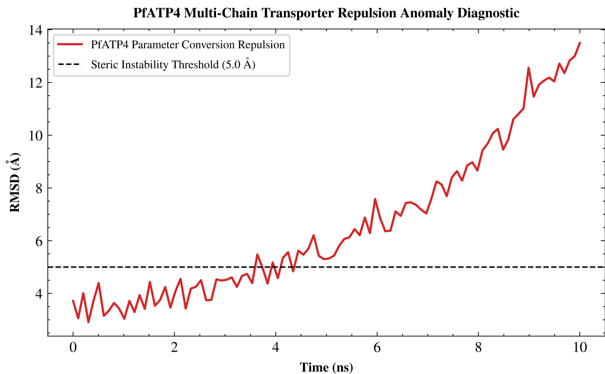
Figure S7: PfATP4 Multi-Chain Transporter Parameter Conversion Repulsion Anomaly Diagnostic. Trajectory RMSD (Å) over 10 ns demonstrating severe steric repulsion introduced by force-field parameter conversion for multi-chain membrane transporters. Rendered using SciencePlots publication styling.
