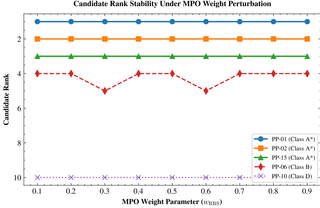
Figure S2: Multi-Parameter Optimization (MPO) Rank Invariance Under Weight Perturbation. Candidate rank trajectories across composite MPO weight variations ( w_{RRS} \in [0.1, 0.9] ). Complete rank stability is maintained for Class-A* leads ( PP-01 , PP-02 , PP-15 ), confirming that candidate prioritization is robust against subjective weighting parameters. Rendered using SciencePlots publication styling.
