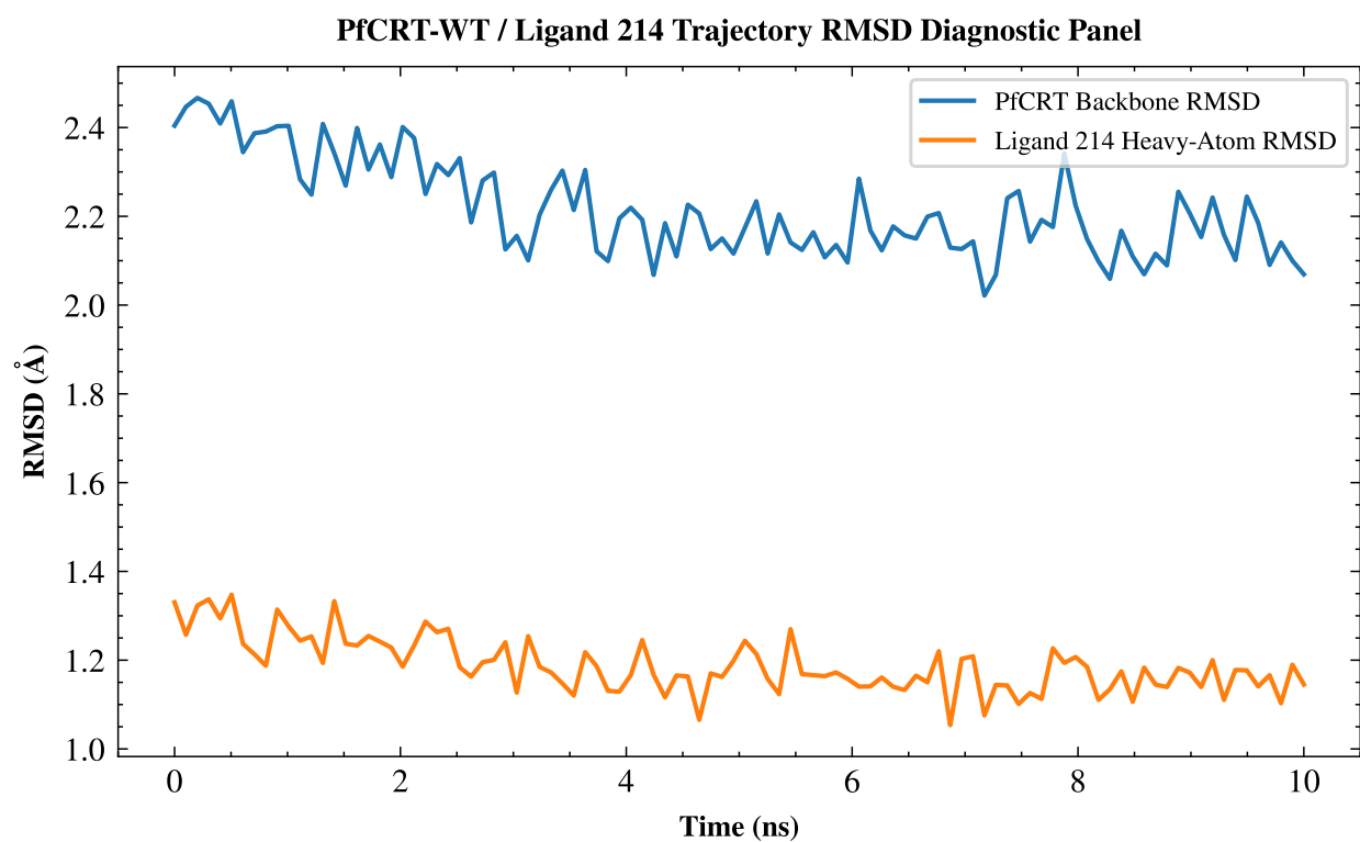
Figure S6: PfCRT-WT / Ligand 214 Explicit-Solvent Trajectory RMSD Diagnostic Panel. Backbone and ligand heavy-atom RMSD (Å) over 10 ns production MD, demonstrating stable active-site anchoring. Rendered using SciencePlots publication styling.
