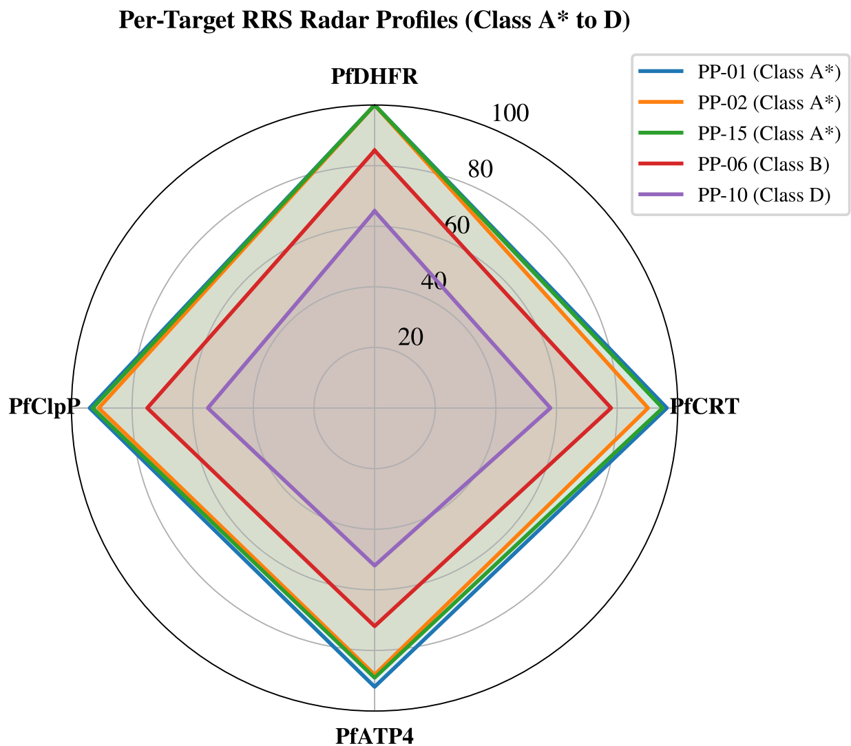
Figure S3: Per-Target Resistance-Resilience Score (RRS) Multi-Dimensional Radar Profiles. Per-target RRS retention profiles across Class A* (resilient leads), Class B (moderate retention), and Class D (penalized). Class-A* leads maintain balanced retention ( \geq 90\% ) across all target axes, whereas Class D candidates suffer target-specific score loss. Rendered using SciencePlots publication styling.
