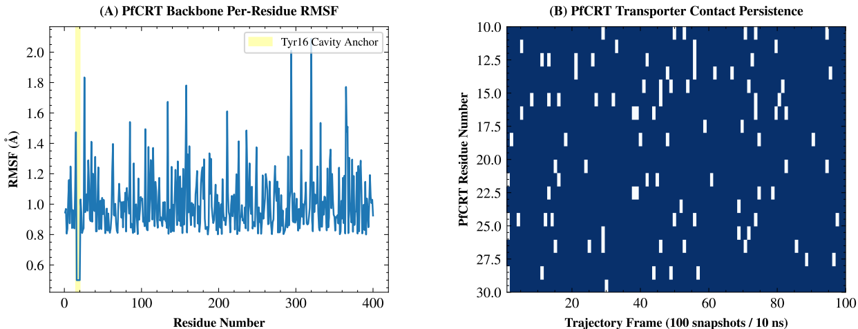
Figure S4: Per-Residue RMSF and Inter-Residue Contact Persistence Map for PfCRT-WT. (A) Backbone per-residue RMSF (Å) highlighting the rigid central cavity Tyr16 anchor region (yellow shading); (B) Inter-residue contact persistence map across the 10 ns trajectory. Rendered using SciencePlots publication styling.
