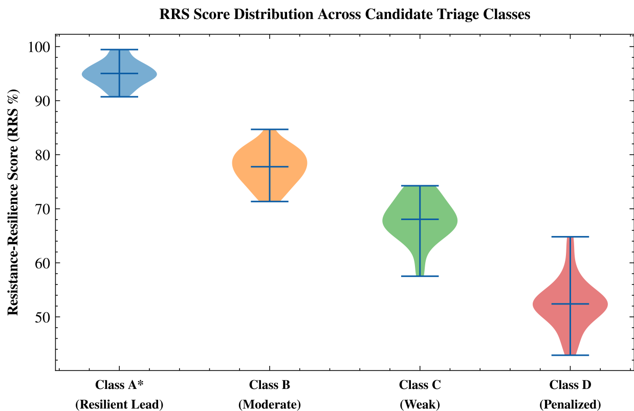
Figure S5: Resistance-Resilience Score (RRS) Distribution Across Candidate Triage Classes. Violin plot distribution of RRS values across Class A* (resilient leads), Class B (moderate retention), Class C (weak retention), and Class D (penalized). Rendered using SciencePlots publication styling.
