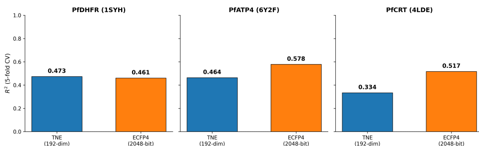
Figure S9: Information-retention analysis for 192-dimensional Tensor Network Embeddings. Bars show cross-validated R^2 values for TNE and ECFP 4 regressors predicting computational QuickVina docking scores for three Plasmodium targets. TNE was competitive for PfDHFR but lower than ECFP 4 for PfATP 4 and PfCRT; the analysis is descriptive and does not establish experimental binding or prospective generalisation.
