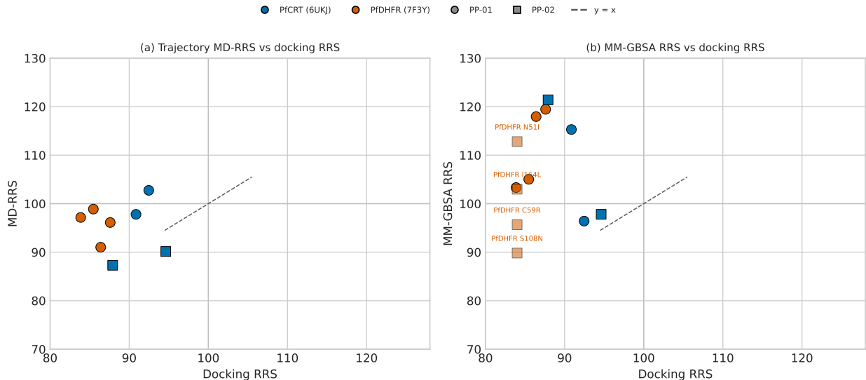
Figure S5: Trajectory-derived ratios versus docking RRS (wild type = 100). (a) Mean minimum-distance ratios for eight mutants with a docking wild-type reference. (b) MM-GBSA ratios versus docking RRS (four PP-02 PfDHFR states lack a docking wild-type reference). The dashed diagonal indicates equality; horizontal and vertical guides denote the wild-type ratio. The two metrics showed opposite operational directions in most matched rows. Neither quantity is a free-energy or experimental resistance measure.
