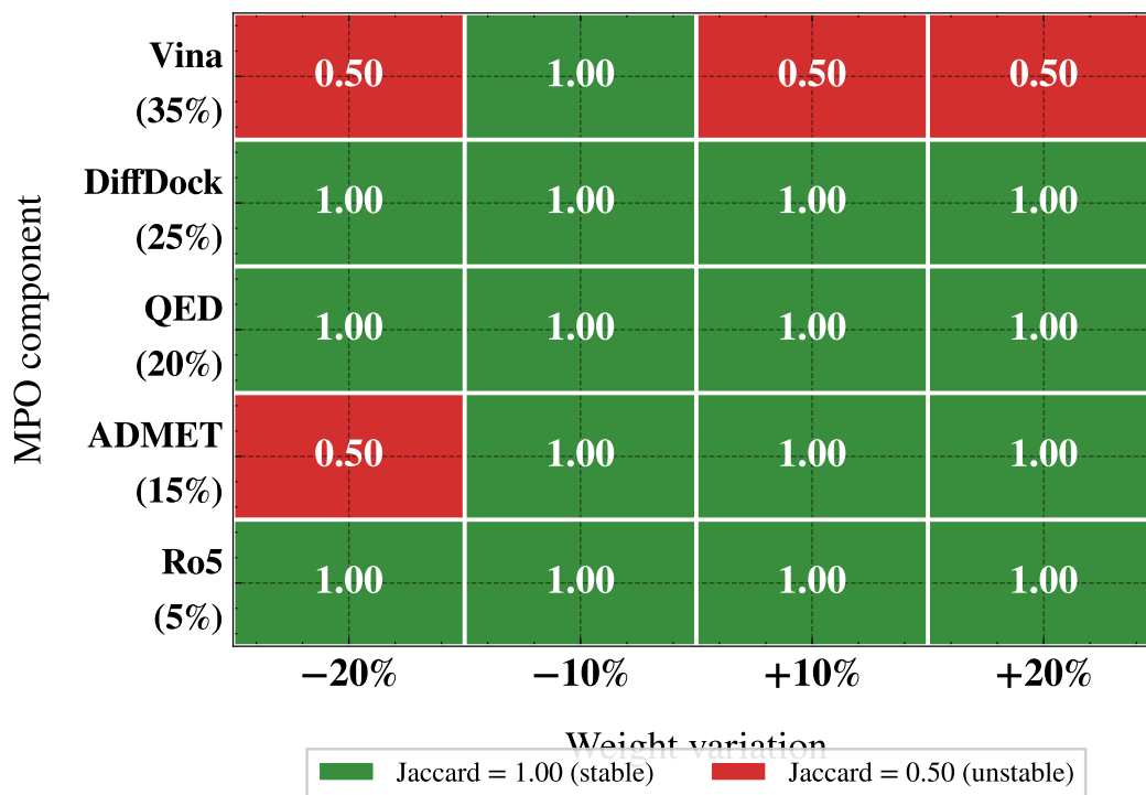
Figure S2: Sensitivity of the top-20 candidate ranking to \pm 20\% perturbation of each MPO weight, measured as Jaccard similarity. Green (1.00) indicates no change; red (0.50) indicates substantial reordering.
