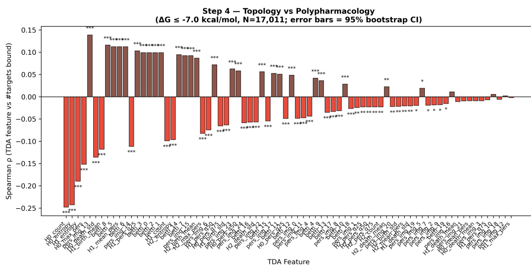
Figure 3.4.7: Topological features against multi-target docking profiles ( N = 17\,011 molecules docked against four P. falciparum targets). Persistence-derived features correlate negatively but weakly with the number of targets meeting the \Delta G \leq -7.0 kcal mol -1 threshold. The endpoint is a docking-derived count, so this is a hypothesis-generating association rather than a mechanistic polypharmacology rule.
