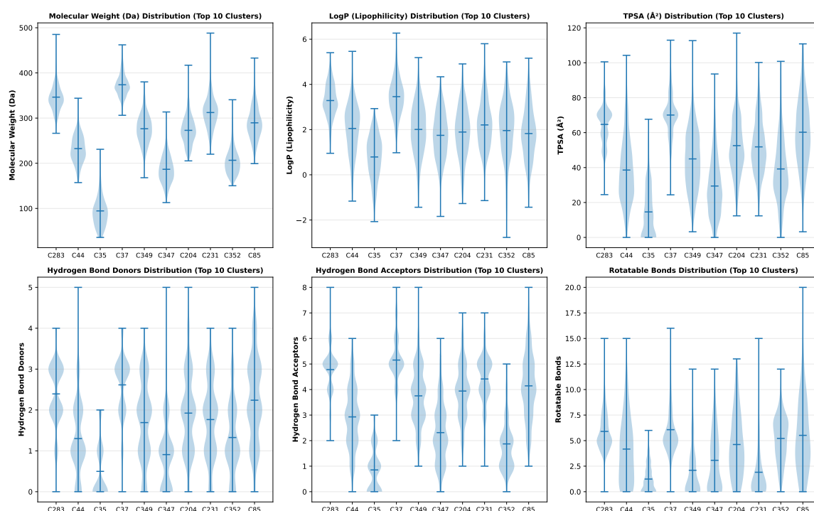
Figure 3.2.6: Physicochemical distributions (lipophilicity, molecular weight and topological polar surface area) across the ten leading clusters of the 484-cluster k -means partition. The property bands overlap strongly between clusters, so centroid-based sampling does not stratify the property space by construction.
