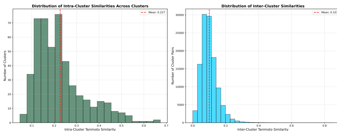
Figure 3.2.5: Tanimoto similarity distributions within clusters (left, mean 0.227, averaged over clusters) and across cluster pairs (right, mean 0.101) of the 484-cluster partition. The roughly 2.2-fold separation supports reading each cluster representative as a structurally coherent sampling unit.
