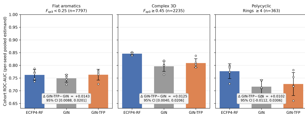
Figure 3.5.2: Performance by structural-complexity cohort in the learned-representation study under the recomputed per-seed estimand (per-seed points, mean \pm SD over five seeds). The GIN–TFP gain over GIN is positive in every cohort, with bootstrap 95% intervals annotated per panel, but it does not increase with structural complexity and the polycyclic interval includes zero. Base GIN shows its largest deficit against ECFP4–RF on the stereochemically rich cohorts.
