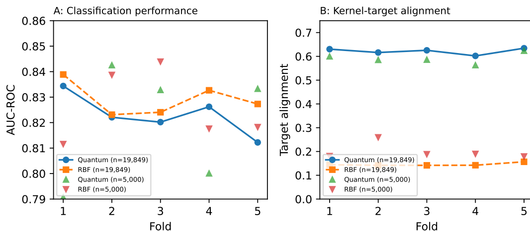
Figure 3.4.5: Quantum kernel benchmark. Panel (A): per-fold AUC for the quantum kernel and the gamma-tuned RBF baseline at n = 19849 and n = 5000 ; the two overlap at every fold. Panel (B): kernel–target alignment per fold, where the quantum kernel reaches 0.622(13) against 0.145(6) for RBF, yet this geometric advantage does not translate into classification performance ( \Delta\text{AUC} = -0.006 ).
