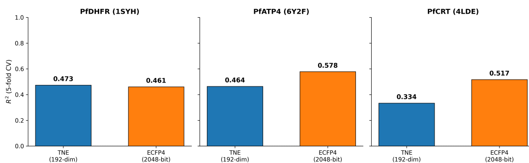
Figure 3.4.4: Cross-validated regression of docking scores on molecular representations. The tensor network embedding is competitive with ECFP4 on PfDHFR but not on the remaining targets. Because embeddings and regression endpoint come from the same molecular set, this quantifies information retention rather than prospective transfer.
