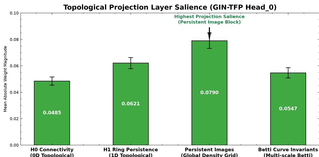
Figure 3.5.3: Mean projection saliency of descriptor blocks in the topological and tensor fusion heads of the learned-representation study. The persistent-image dimensions carry the largest mean weight magnitude, yet the corresponding aggregate scaffold-split gain remains 0.0091 AUC points, so saliency is not evidence of predictive contribution.
