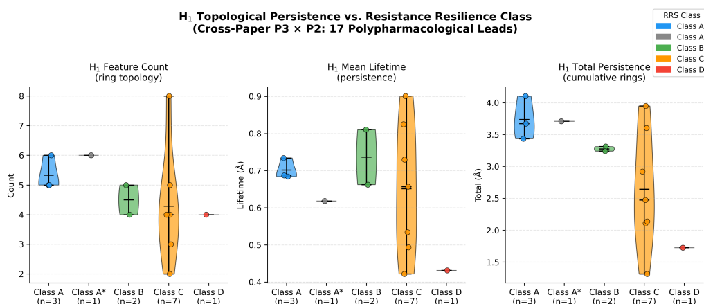
Figure 3.4.8: Distribution of H_1 cycle persistence across resistance-resilience classes. The apparent association between topological complexity and resistance resilience is size-mediated and does not survive control for molecular size and structural covariates, so H_1 persistence is not an independent topological predictor of the resistance-resilience score.
