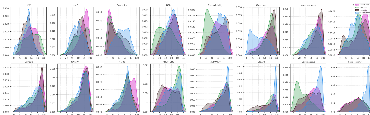
Figure 3.2.7: Predicted ADMET and toxicity endpoint distributions stratified by compound source (synthetic antimalarials, African natural products, similarity-search analogues and SELFIES variants), from the machine-learning platform used for the prioritisation composite [99] . The endpoints feed the ADMET term of the multi-parameter score and are used for ranking only.
