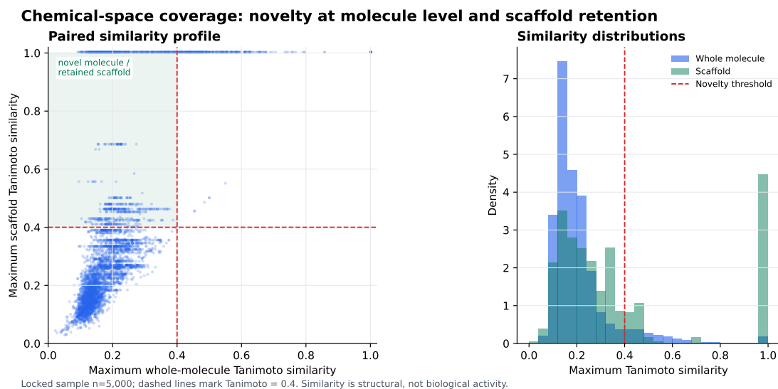
Figure 3.2.1: Coverage of the hybrid library relative to the African natural-product seed set. Whole-molecule novelty (92.6 % of a 5000-molecule sample below a Tanimoto similarity of 0.4) coexists with scaffold retention (69.3%; 70 of 101 annotated seed scaffolds). The gap between whole-molecule and scaffold similarity distributions defines the scaffold paradox analysed topologically in the representation study.
