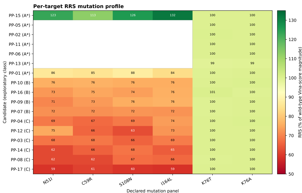
Figure 3.2.10: Per-target mutation-resilience profiles for the Set-C cohort. Values are ratios of Vina-score magnitudes relative to the declared wild-type denominator; blank cells mark wild-type non-binders excluded from the denominator. The classes are computational operational categories, not biological resistance phenotypes.
