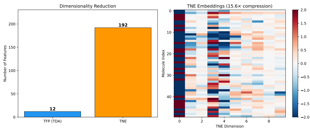
Figure 3.4.3: Compression behaviour of the Tucker tensor network embedding. The 192-element core retains docking-score-predictive information on the derivation panel, reaching R^2 = 0.473 for PfDHFR against 0.461 for ECFP4, while ECFP4 remains stronger for PfATP4 and PfCRT. Reconstruction error increases for structurally atypical molecules, so compression quality is chemical-space dependent.
