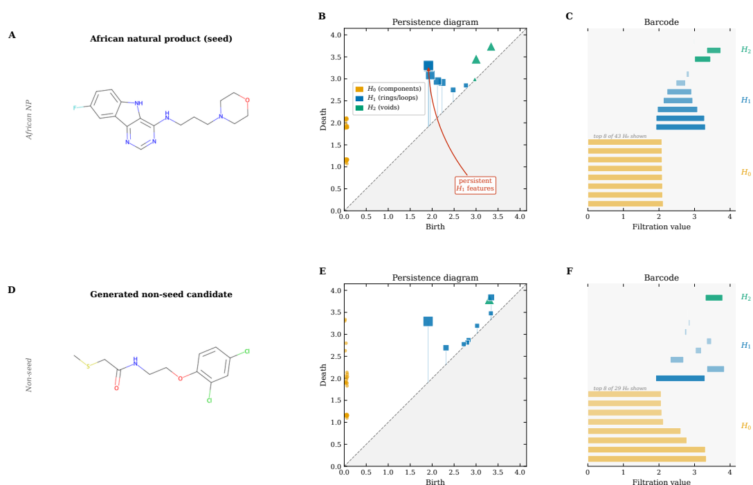
Figure 3.4.2: Representative persistence diagrams underlying the topological fingerprint. Vietoris–Rips persistence was computed up to homology dimension two on weighted molecular graphs whose edge weights are w_{ij} = d_{ij}(1 + Z_i Z_j / 100) , so that interactions involving heavier atoms contribute more strongly. The primary activity analysis uses a 78-feature vector combining homology summaries, persistence-image and Betti-curve components.
