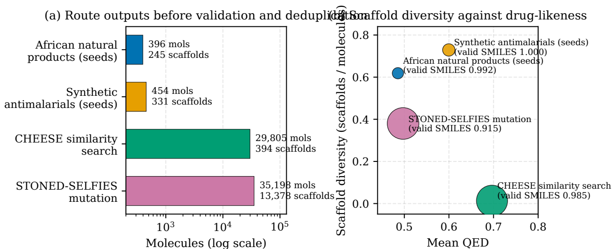
Figure 3.2.2: Composition of the two expansion routes against their seed sets, counted before validation and deduplication. (a) Route outputs on a logarithmic scale with unique Bemis–Murcko scaffold counts. (b) Scaffold diversity against mean QED, with point area proportional to library size and valid-structure fractions annotated. The similarity-search route is drug-like but scaffold-narrow (29805 molecules, 394 scaffolds); the SELFIES route is scaffold-diverse at a QED cost (35198 molecules, 13378 scaffolds).
