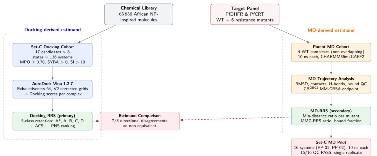
Figure 3.3.1: Integrated resistance-aware polypharmacology and molecular-dynamics triage framework of the resistance-scoring study. Static multi-target docking feeds the resistance-resilience score, the African-chemotype structural index and the polypharmacology network similarity; 10 ns explicit-solvent molecular dynamics then runs as a secondary structural check. Docking-derived and trajectory-derived quantities are distinct estimands and are never combined into a single score.
