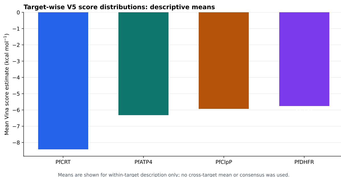
Figure 3.2.9: Target-wise docking profile of the 17-member Set-C cohort. Because AutoDock Vina scores are not calibrated across dissimilar pockets, breadth is summarized as the count of targets at or below each target's within-cohort median rather than as a cross-target average. The within-target threshold is a prioritization device, not an affinity cutoff.
