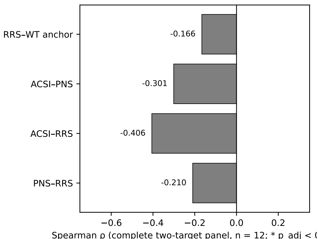
Figure 3.3.4: Cross-metric Spearman correlations on the complete two-target set ( n = 12 ): PNS-RRS \rho = -0.2098 , ACSI-RRS \rho = -0.4056 , ACSI-PNS \rho = -0.3007 and RRS-weakest-WT-anchor \rho = -0.1661 ; none is significant after Bonferroni correction (adjusted p \geq 0.51 ; 100 000 permutations, seed 42). The absence of significant inter-metric association is consistent with distinct ranking dimensions rather than redundant signals. With 12 observations these intervals are wide and the tests are descriptive.
