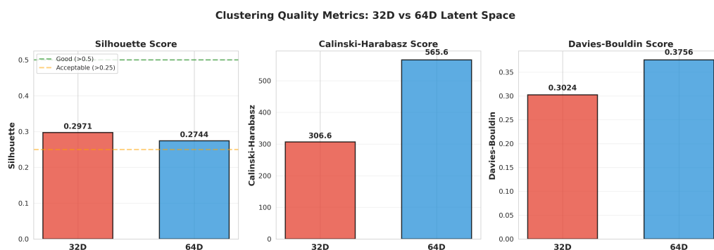
Figure 3.2.4: Clustering-quality diagnostics of the k -means partitions of the 32- and 64-dimensional latent spaces: silhouette score, Calinski–Harabasz index and Davies–Bouldin index. The comparison is mixed—32D leads on silhouette and Davies–Bouldin, 64D on Calinski–Harabasz—which motivated the selection of the 64-dimensional space on the separation criterion.
