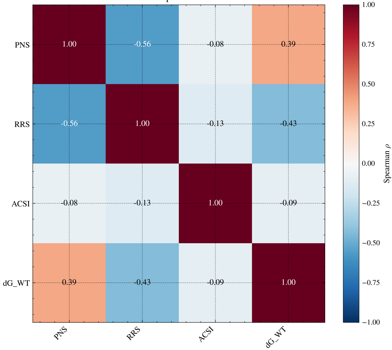
Cross-Metric Spearman Correlations
