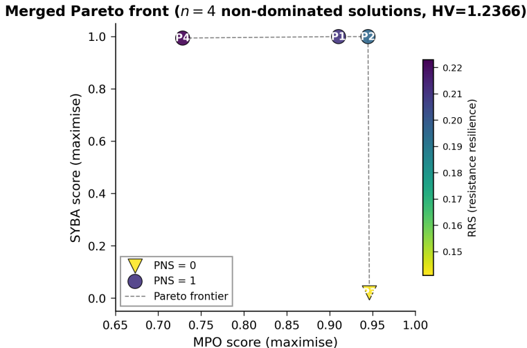
Figure 3: Canonical merged Pareto front from 20 independent Pareto-MCTS seeds. Marker shape encodes the polypharmacology-network score (PNS); colour encodes the resistance-resilience score (RRS). The four solutions are mutually non-dominated across the active objectives MPO, SYBA, RRS and PNS; SA is constant at 3.0 and excluded from the dominance check and the hypervolume. Data: results/pareto/merged_pareto_front.csv.
