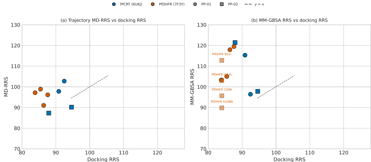
Figure S5: Trajectory-derived ratios versus docking RRS (wild type = 100). (a) Mean minimum-distance ratios for eight mutants with a docking wild-type reference. (b) MM-GBSA ratios versus docking RRS (four PP-02 PfDHFR states lack a docking wild-type reference). The dashed diagonal indicates equality; horizontal and vertical guides denote the wild-type ratio. The two metrics showed opposite operational directions in most matched rows. Neither quantity is a free-energy or experimental resistance measure.
