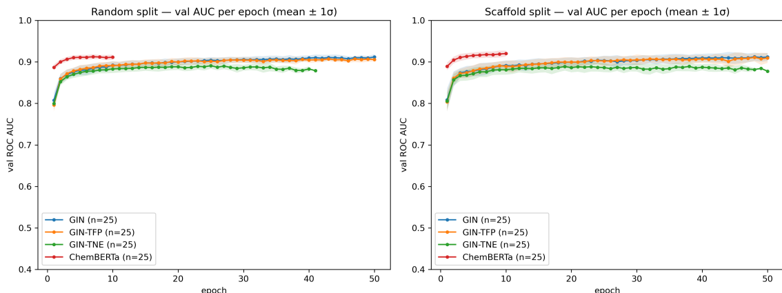
Figure 2: Validation ROC AUC trajectory over training epochs across all models under random and scaffold splits. Early stopping with patience 10 selects the optimal validation checkpoint prior to test evaluation across five folds repeated over five seeds (25 fold-seed replicates per split).
