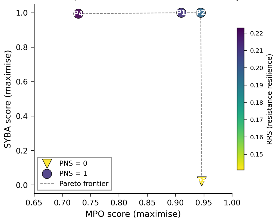
Figure 3: Canonical Pareto front obtained by merging 20 independent Pareto-MCTS seeds and removing dominated solutions. Four non-dominated molecules remain ( HV = 1.2366 ). The 2D projection shows MPO versus SYBA; point colour encodes the Resistance Resilience Score (RRS), and marker shape encodes the Polypharmacology Network Score (PNS): circles (PNS = 1) and triangles (PNS = 0). All four solutions share SA=3.0 .
