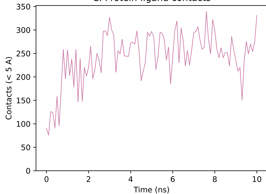
C. Protein-ligand contacts
