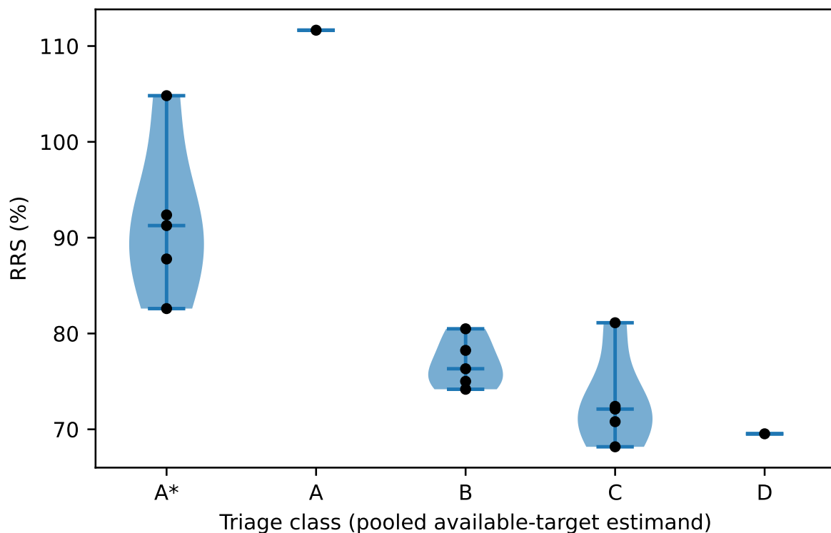
Figure S5: RRS distribution across triage classes. Violin plot of per-candidate RRS (pooled available-target estimand, c_rrs_classification.csv ) for Classes A* ( n = 5 ), A ( n = 1 ), B ( n = 5 ), C ( n = 5 ), and D ( n = 1 ); black points show individual candidates.
