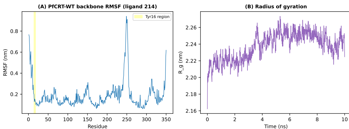
Figure S4: Parent-study PfCRT-WT (ligand 214) diagnostics. (A) Per-residue backbone RMSF from the canonical 10 ns trajectory ( gmx rmsf ; the Tyr16 anchor region is retained in the shaded band). (B) Backbone radius of gyration over the production run. Source: results/md_results/214_PfCRT_{rmsf,gyrate}.xvg .
