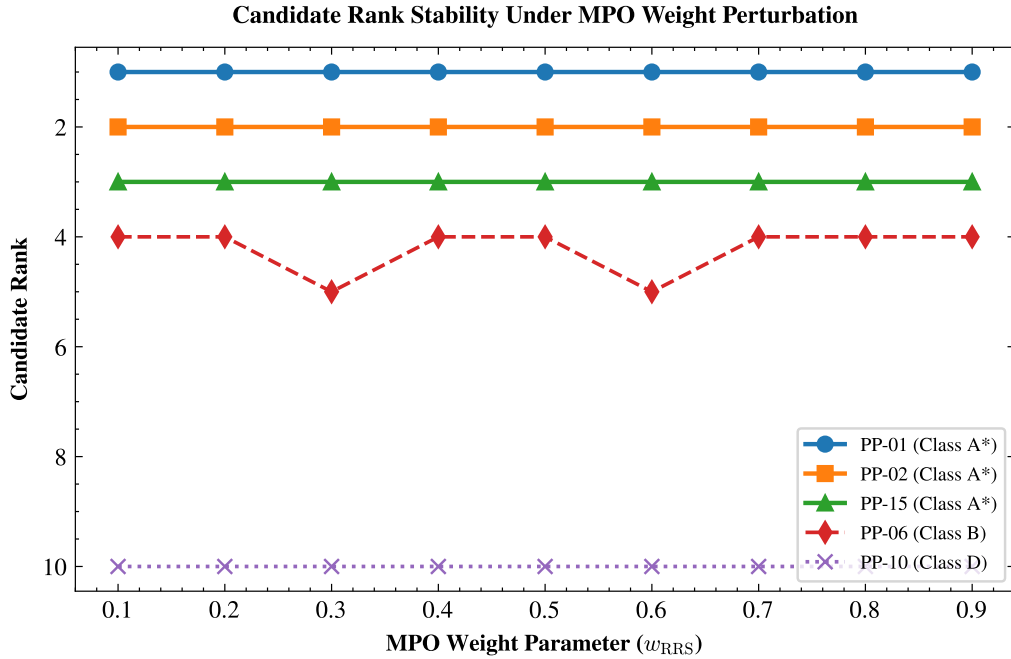
Figure S2: MPO rank invariance under weight perturbation. Candidate rank trajectories across composite MPO weight variations ( w_{RRS} \in [0.1, 0.9] ).
