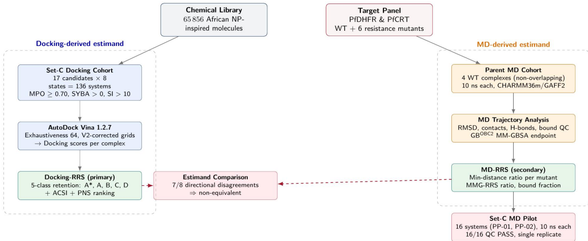
Figure 1: Study design. Docking-derived RRS, ACSI, and PNS are computed on the 17 Set-C candidates across 136 WT/mutant PfDHFR and PfCRT systems. Four upstream-cohort complexes (non-overlapping with the Set-C list) undergo a single 10 ns production MD per system (CHARMM36m/GAFF2 or OpenFF/CHARMM36m for the upstream and Set-C cohorts, respectively); a 16-system Set-C pilot (PP-01 and PP-02, single 10 ns replicate per state) is reported separately and does not define the RRS classes. None of the MD trajectories is replicated at the level recommended by the JCIM MD-reporting guidelines 17 . The shared candidate and workflow provenance means that the upstream cohort is contextual rather than an independent validation dataset.
