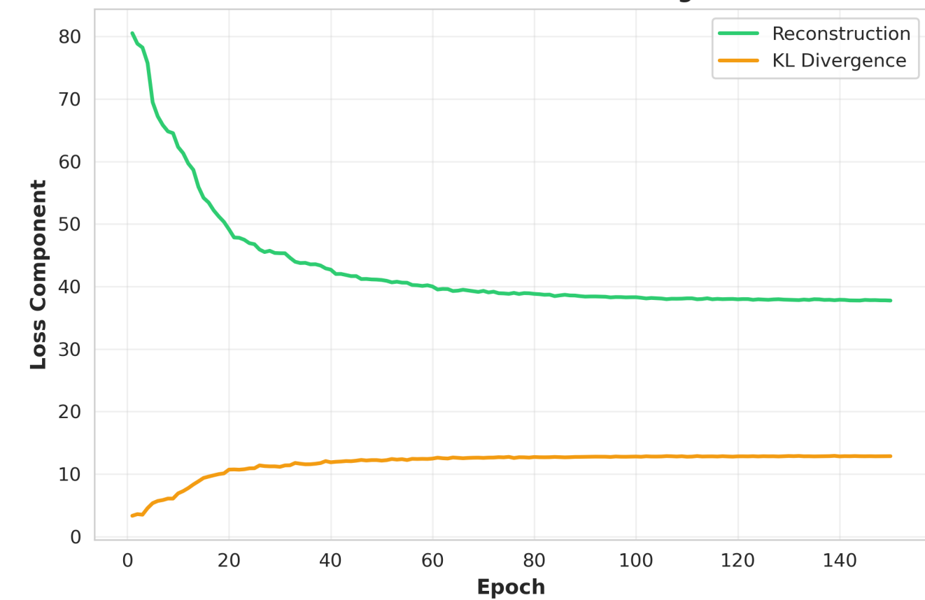
64D: Reconstruction vs KL Divergence
