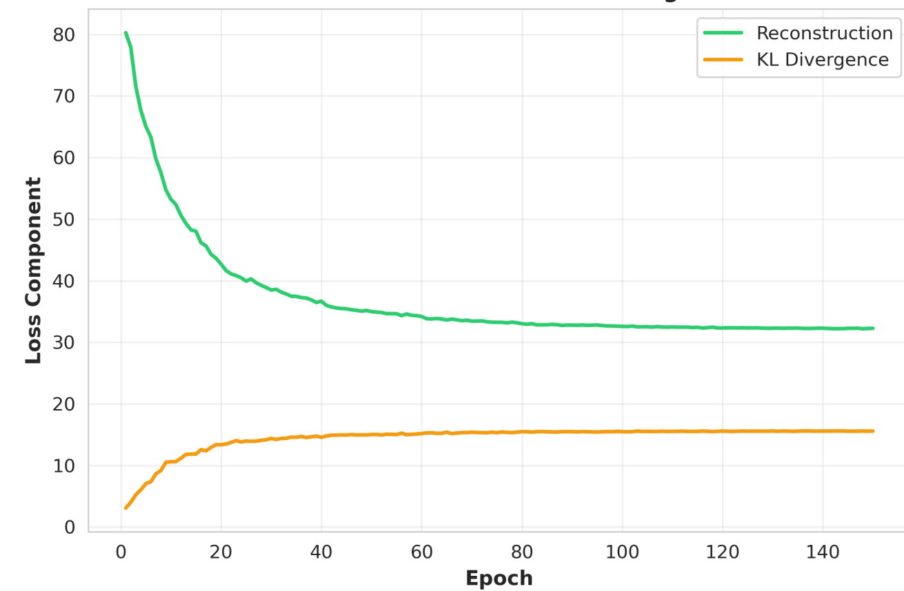
32D: Reconstruction vs KL Divergence
