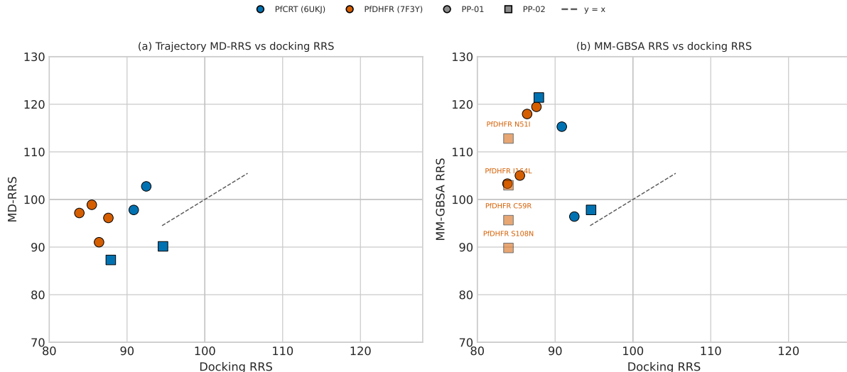
Figure 4: Set-C MD pilot trajectory-derived RRS estimates versus docking RRS (WT-normalised, WT = 100). Panel (a): MD-RRS (mean-minimum-distance geometry) versus docking RRS for the eight mutant systems with both estimates; panel (b): MM-GBSA RRS versus docking RRS, with the four PP-02 PfDHFR systems (no docking WT reference in the pilot) shown on the MM-GBSA axis only. Points are coloured by target (PfCRT, blue; PfDHFR, orange) and shaped by candidate (PP-01, circle; PP-02, square). Docking predicted looser mutant binding for all systems (RRS < 100); the trajectory-derived estimates do not reproduce this pattern. Secondary, exploratory analysis; no primary claim is based on it.
