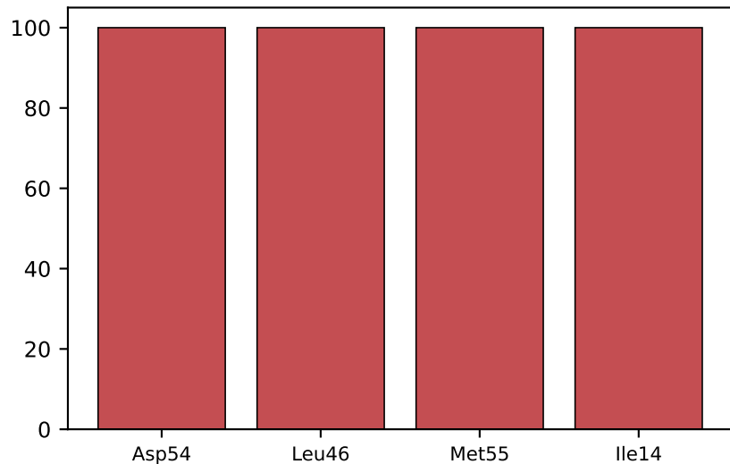
(B) PfDHFR hotspot contacts (max across systems)
