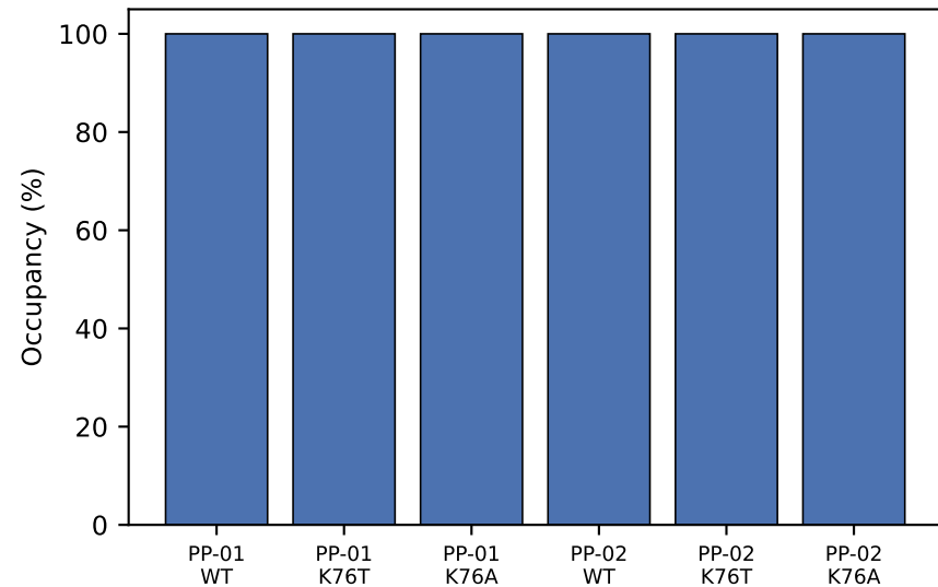
(A) PfCRT Tyr16 contact occupancy
