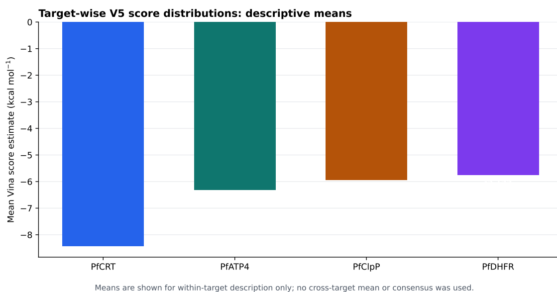
Figure 2: Descriptive target-wise means from the raw docking panel. Bars show the within-target mean across the 17 candidates. Means are shown only within target; no cross-target arithmetic mean or consensus score was used. These summaries are computational scoring-function outputs, not experimental affinity measurements.
