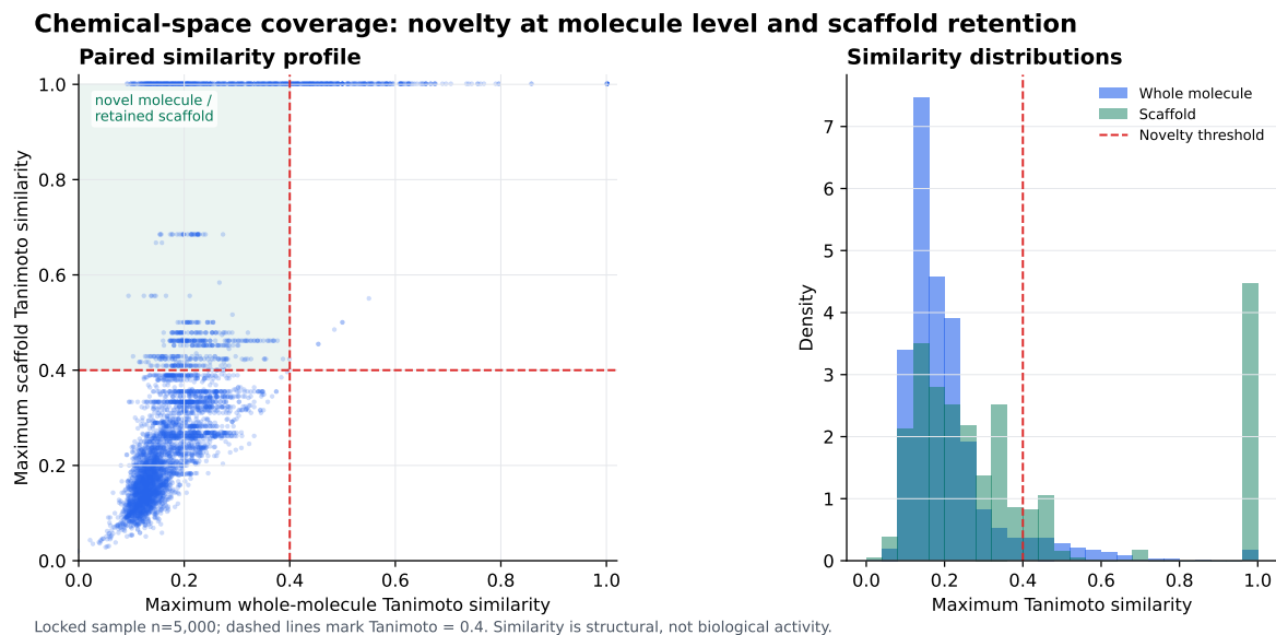
Figure 1: Chemical-space coverage in the 5 000-molecule novelty-analysis sample. The paired plot compares maximum whole-molecule and scaffold Morgan-fingerprint Tanimoto similarities to the African-natural-product reference set; the dashed lines mark the operational threshold of 0.4. The upper-left region represents molecules that are dissimilar at the whole-molecule level while retaining scaffold-level similarity. Similarity is a structural descriptor and does not indicate biological activity, target preference, or synthetic success.
