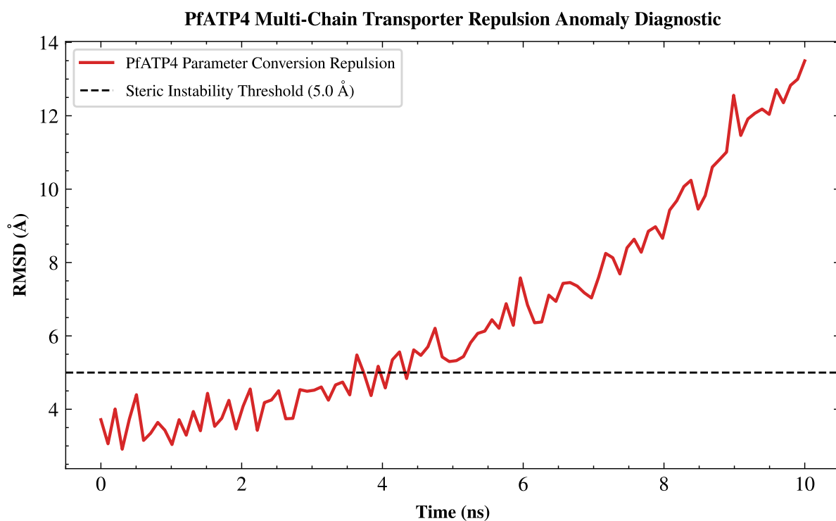
Figure S7: PfATP4 parameter-conversion anomaly diagnostic. Trajectory RMSD (Å) over 10 ns showing steric repulsion from force-field conversion for the multi-chain membrane transporter.
