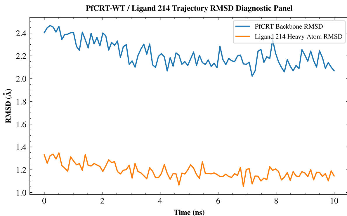
Figure S6: PfCRT-WT / Ligand 214 trajectory RMSD diagnostics. Backbone and ligand heavy-atom RMSD (Å) over 10 ns production MD.
