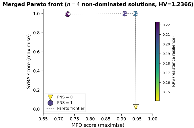
Figure 2: Canonical merged Pareto front from 20 independent Pareto-MCTS seeds. Marker shape encodes the polypharmacology-network score (PNS); colour encodes the resistance-resilience score (RRS). The four solutions are mutually non-dominated across the active objectives MPO, SYBA, RRS and PNS; SA is constant at 3.0 and excluded from the dominance check and the hypervolume. Data: results/pareto/merged_pareto_front.csv.
