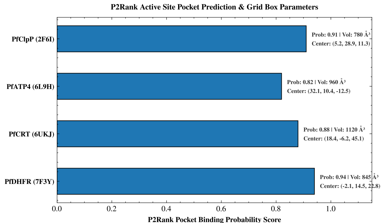
Figure S1: P2Rank pocket prediction vs. Vina grid-box alignment. Pocket probability scores and volumes ( \text{\AA}^3 ) for PfDHFR (7F3Y, prob 0.94, vol 845 \text{\AA}^3 ), PfCRT (6UKJ, prob 0.88, vol 1120 \text{\AA}^3 ), PfATP4 (6L9H, prob 0.82, vol 960 \text{\AA}^3 ), and PfClpP (2F6I, prob 0.91, vol 780 \text{\AA}^3 ).
