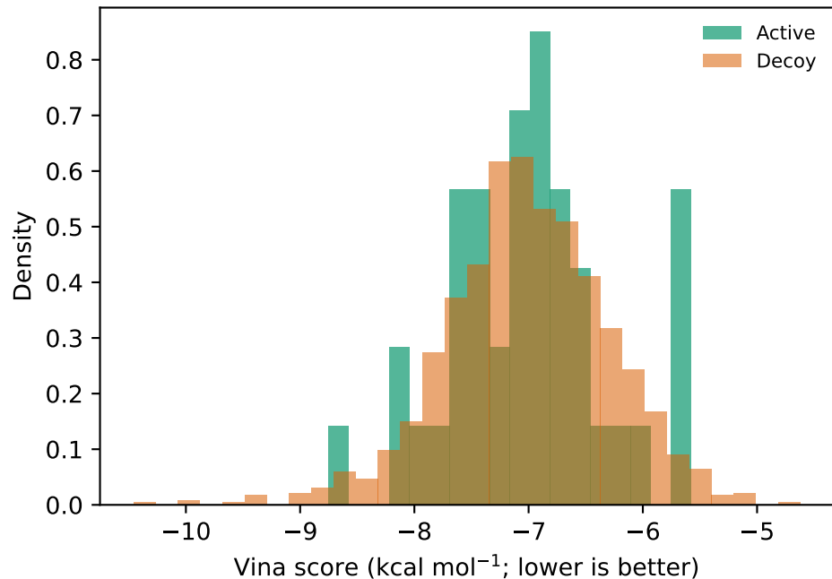
Score distributions
