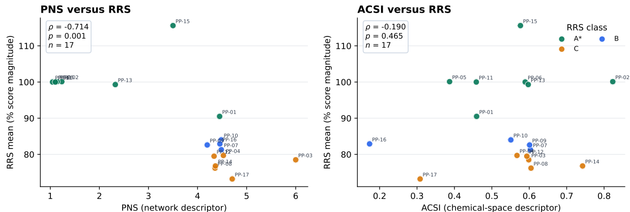
Figure 2: Exploratory relationships between RRS and PNS or ACSI. Points are colored by the operational RRS class. These associations are descriptive source-panel analyses and do not establish causality, biological activity, or resistance protection.
