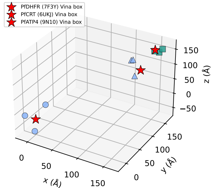
(b) Vina box centers (*) and top-3 P2Rank pockets per receptor (same frame pairs)
