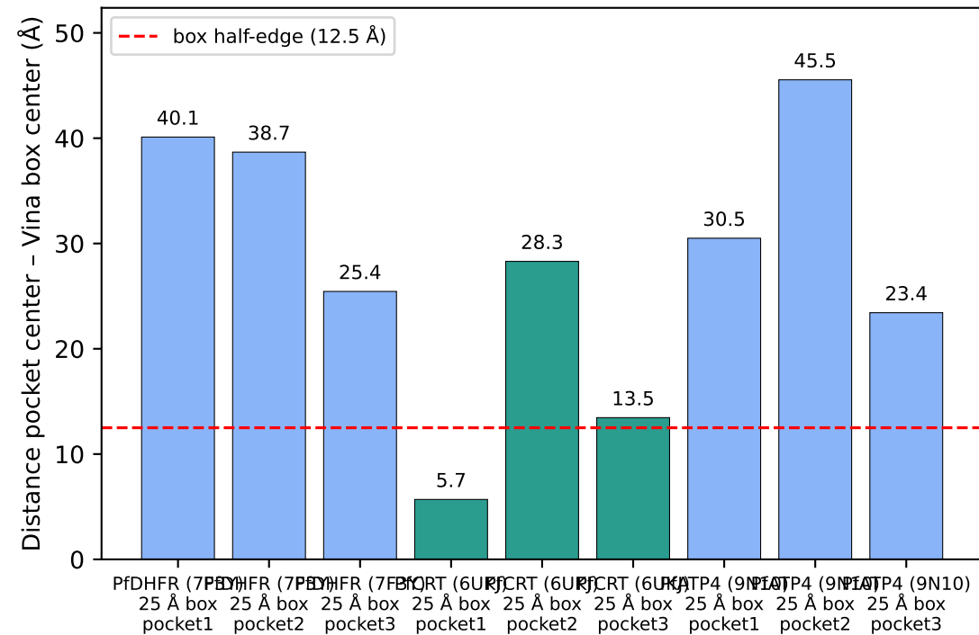
(a) P2Rank pocket centers vs Vina box centers
