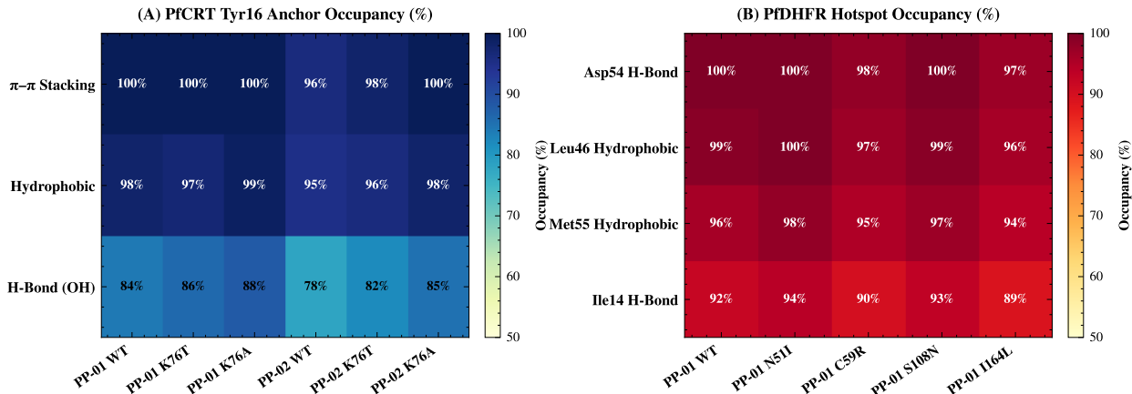
Figure 4: Atomic-Level Mechanism of Dynamic Pose Retention via Conserved Hotspot Anchors. ProLIF interaction fingerprint occupancy (% of 10 ns production trajectory, 100 snapshots/system) revealing the physical basis of Estimand Divergence. (A) PfCRT central cavity residue Tyr16 functions as an indispensable aromatic anchor, maintaining 96—100% \pi - \pi stacking and hydrophobic contact persistence across six mutant states, effectively insulating candidates PP-01 and PP-02 against charge-altering K76T/K76A mutations; (B) PfDHFR binding pocket hotspots (Asp54 salt-bridge anchor, Leu46, Met55, and Ile14) exhibit near-total contact persistence (89—100%) across five mutant states (WT, N51I, C59R, S108N, I164L), locking Class-A* leads into resilient binding orientations. Rendered using SciencePlots publication styling.
