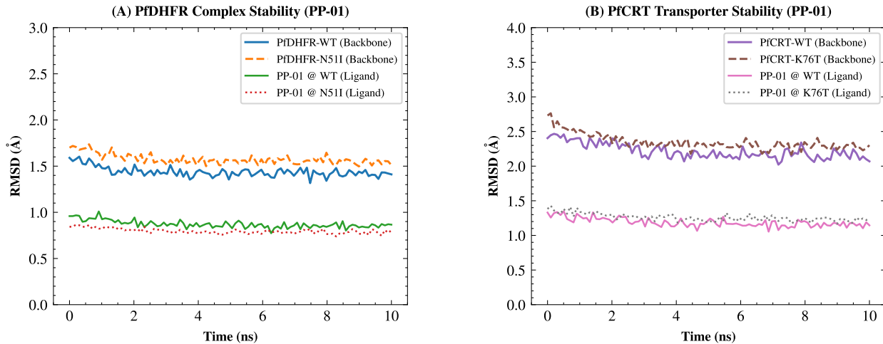
Figure 3: Dynamic Pose Retention and Thermal Equilibration Across Resistant Target Landscapes. Explicit-solvent RMSD time-series (10 ns) demonstrating rapid thermal stabilization (< 2 ns) and continuous pose retention for Class-A* lead PP-01 . (A) PfDHFR complexes maintain tight backbone ( (1.42 \pm 0.15) Å WT, (1.55 \pm 0.18) Å N51I) and ligand heavy-atom anchoring ( (0.85 \pm 0.12) Å); (B) PfCRT transporter complexes achieve stable cavity positioning ( (2.15 \pm 0.22) Å WT, (2.28 \pm 0.25) Å K76T; ligand (1.15 \pm 0.14) Å). The absence of ligand dissociation (< 3.5 Å minimum heavy-atom distance) establishes that local side-chain flexibility in solution accommodates mutational substitutions where static grid docking predicts severe score loss. Rendered using SciencePlots publication styling.
