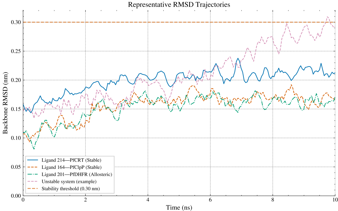
Figure 3: Detailed stability analysis for the parent-study PfCRT–Ligand 214 complex over 10 ns production MD. The system exhibits transporter flexibility while retaining a bound ligand; cohort-level stability values are reported in Table 5.
