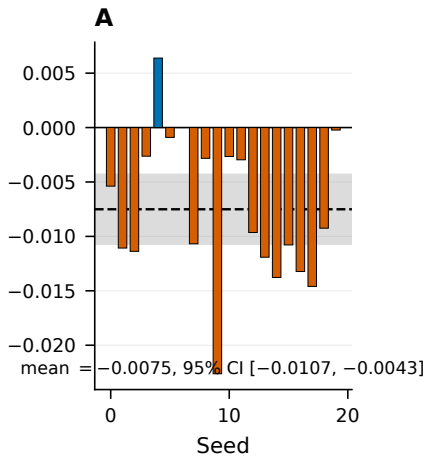
MCTS – random reward
