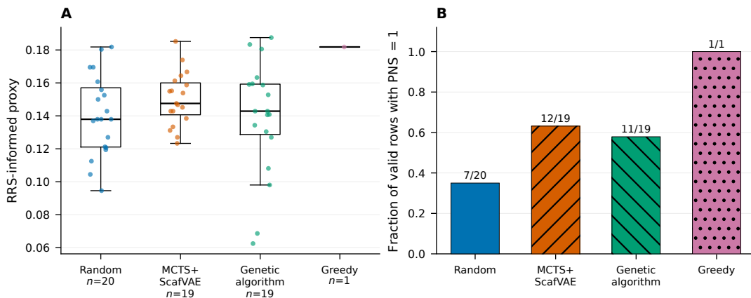
Figure S1: RRS-informed chemotype-similarity and PNS-informed docking-proxy profiles for recorded best-in-seed molecules. Points show individual observations and box summaries. The PNS panel reports the fraction of valid rows with PNS equal to 1.0; intermediate values are retained in the underlying data.
