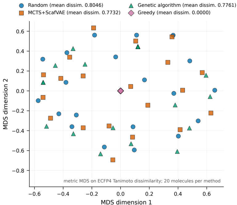
Figure S2: Metric multidimensional-scaling projection of the recorded best-in-seed molecule sets using ECFP4 Tanimoto dissimilarity. Each method contributes 20 molecules. Greedy search collapses to one point because it returns the same local optimum for every seed.
