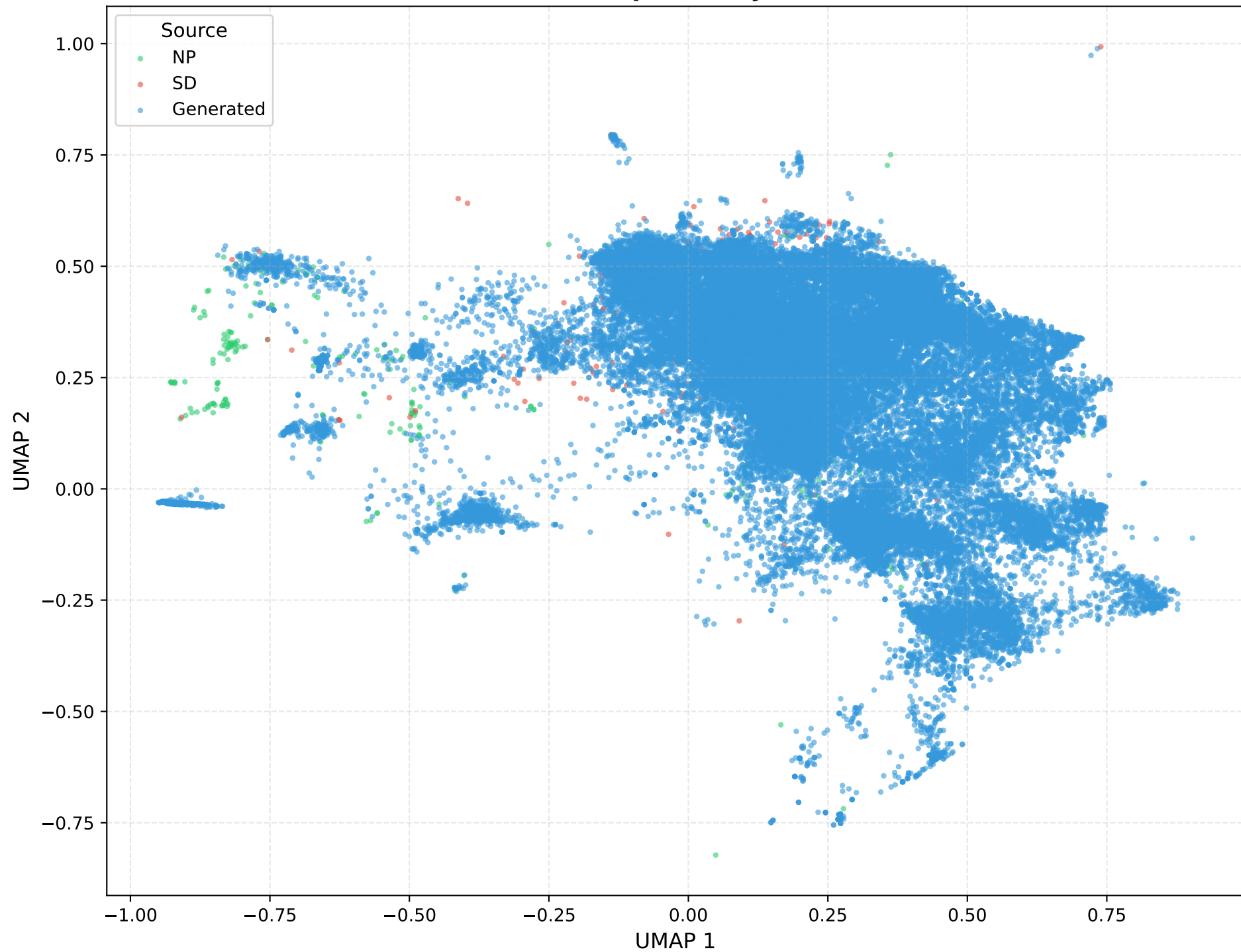
64D VAE Latent Space Projection (UMAP)
