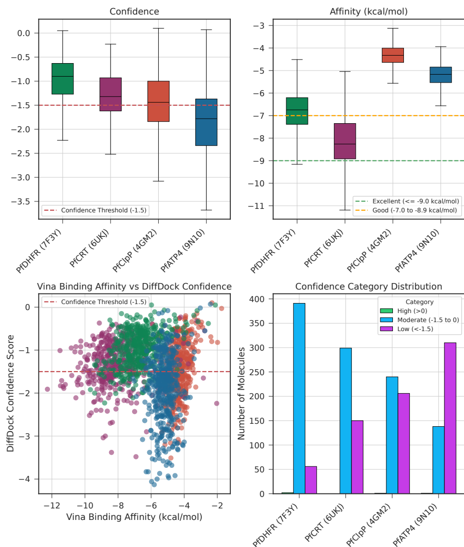
Figure 2: Bivariate consensus docking distributions across four Plasmodium falciparum targets: PfClpP (PDB: 4GM2), PfCRT (PDB: 6UKJ), PfDHFR-TS (PDB: 7F3Y), and PfATP4 (PDB: 9N10). 484 ligand centroids representing 65 856-molecule library screened per target. Compounds stratified into performance tiers: EXCELLENT (best score \leq -7.0 kcal mol ^{-1} and DiffDock confidence \geq 0.0 , red), GOOD ( -7.0 kcal mol ^{-1} to -5.0 kcal mol ^{-1} and DiffDock \geq -1.5 , orange), and OTHERS (grey). Y-axis: DiffDock confidence scores. PfCRT: 85.8 % hit rate; PfClpP: minimal enrichment. Classification thresholds calibrated against ChEMBL antimalarial actives (median -6.9 kcal mol ^{-1} , IQR -7.4 kcal mol ^{-1} to -6.6 kcal mol ^{-1} ; n = 37 ).
