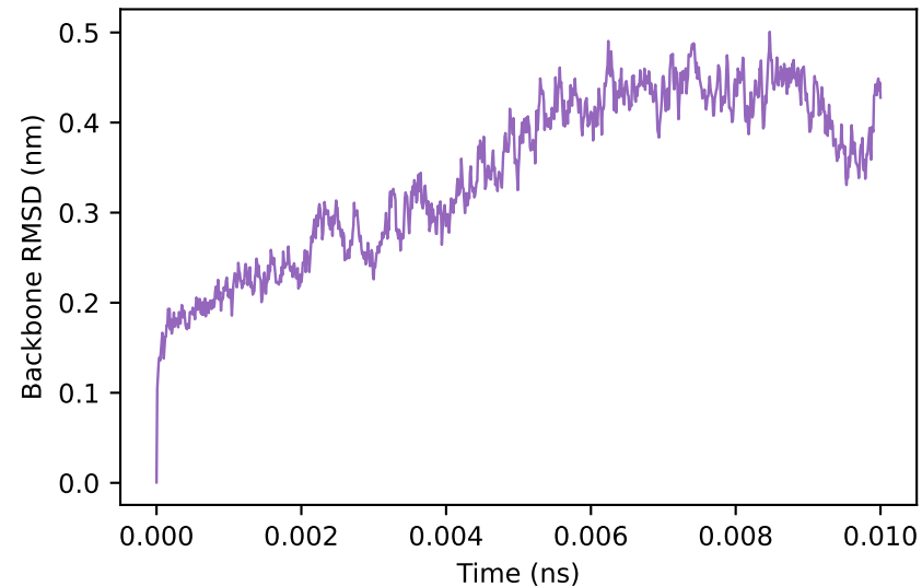
PfCRT-WT (ligand 214)
