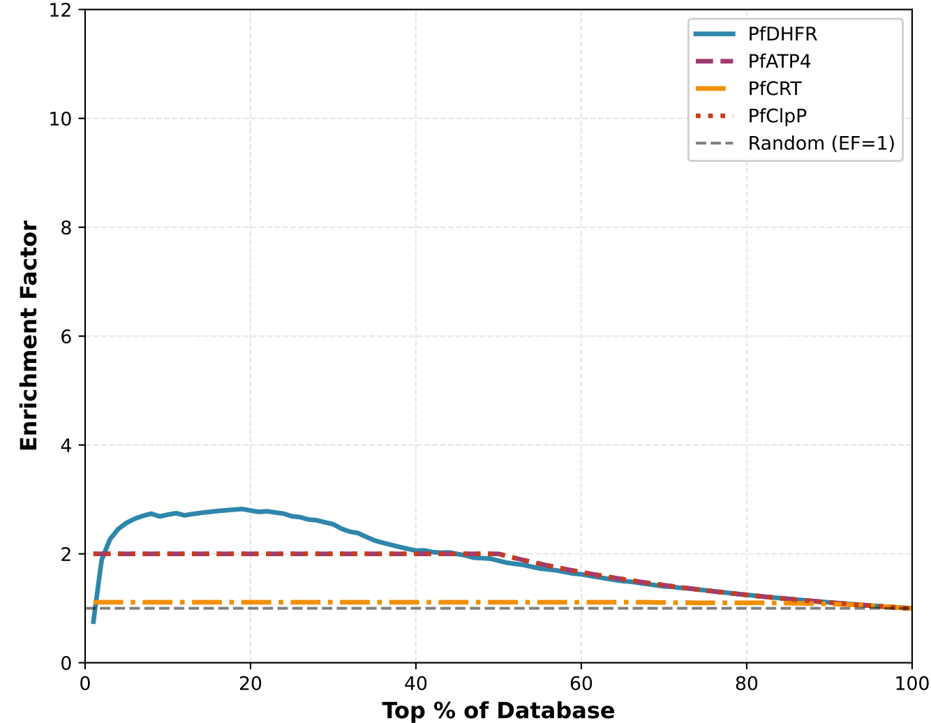
C. Enrichment Factor vs Database Fraction
