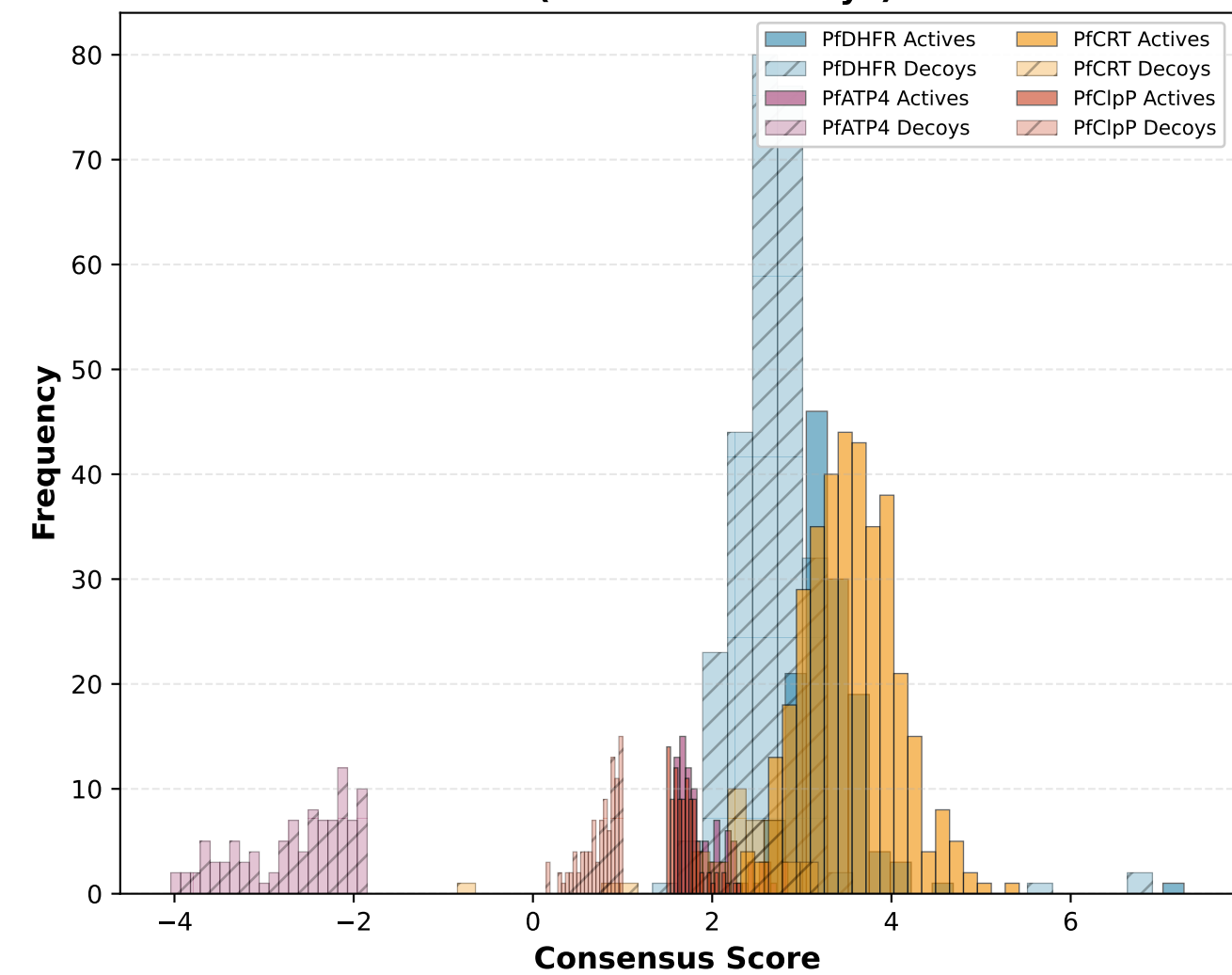
D. Score Distributions (Actives vs Decoys)
