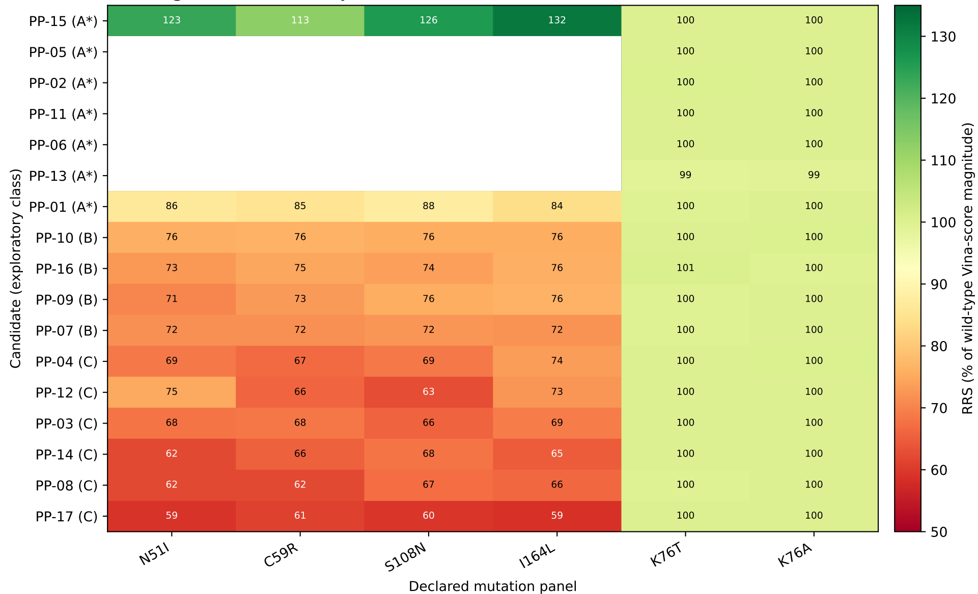
Per-target RRS mutation profile
