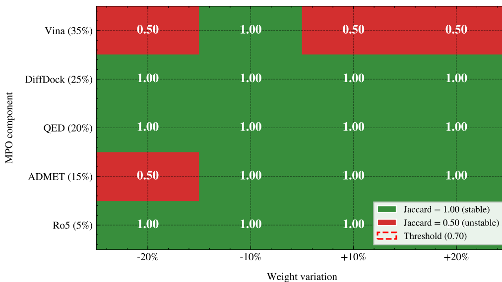
Figure 1: MPO sensitivity analysis heatmap. Each cell shows the Jaccard similarity of the top-20 hit list when the corresponding MPO weight is varied by \pm 20\% . Green (1.00) indicates the hit list is unchanged; red (0.50) indicates substantial reordering.
