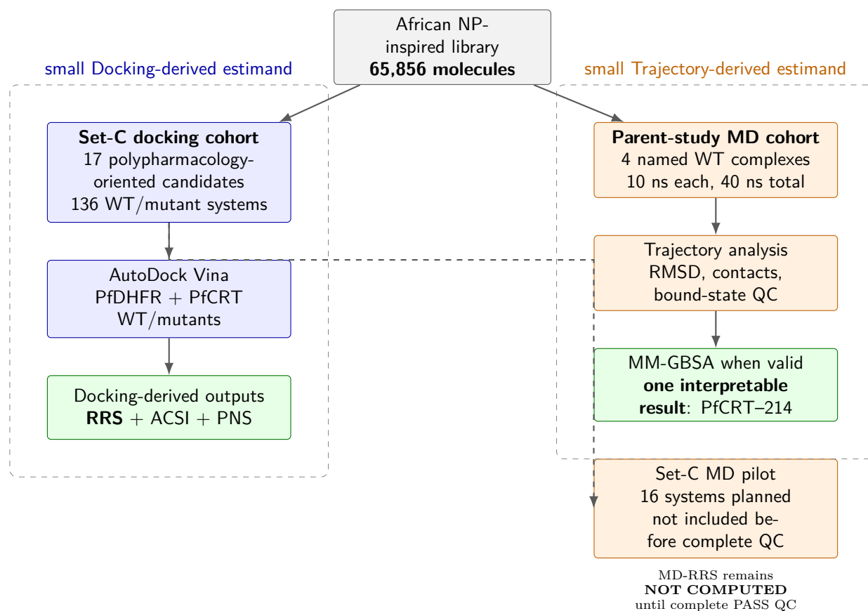
Figure 1: Study design and separation of computational estimands. The 17-member Set-C cohort supports docking-derived RRS, ACSI, and PNS analyses, whereas the four parent-study complexes support a separate targeted MD and MM-GBSA check. The incomplete Set-C MD pilot is not promoted as a result.
