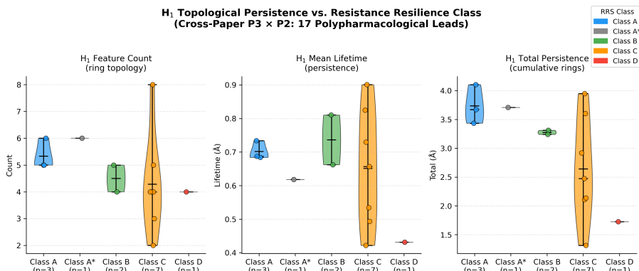
Figure 2: Joint topological analysis linking TFP features with computational resistance-resilience scores. The violin plot is retained as an exploratory illustration of the earlier pilot subset; it is not used as evidence for an independent class effect. In the canonical expanded cohort ( n = 494 ), H_1 count showed a weak unadjusted association with RRS (Spearman \rho = 0.2399 , p = 6.76 \times 10^{-8} ), which was null after adjustment for molecular weight, ring count, fraction sp^3 , and H_0 count ( \rho_{\text{partial}} = 0.0329 , p = 0.4668 ). The association is therefore size-mediated and hypothesis-generating, not evidence of an independent topological predictor.
