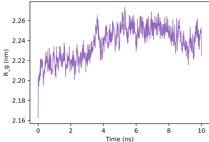
(B) Radius of gyration
