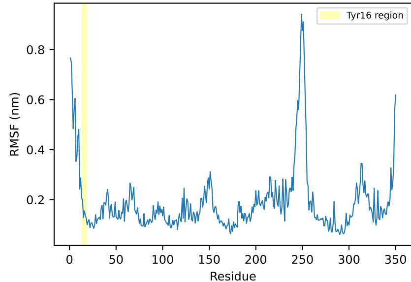
(A) PfCRT-WT backbone RMSF (ligand 214)
