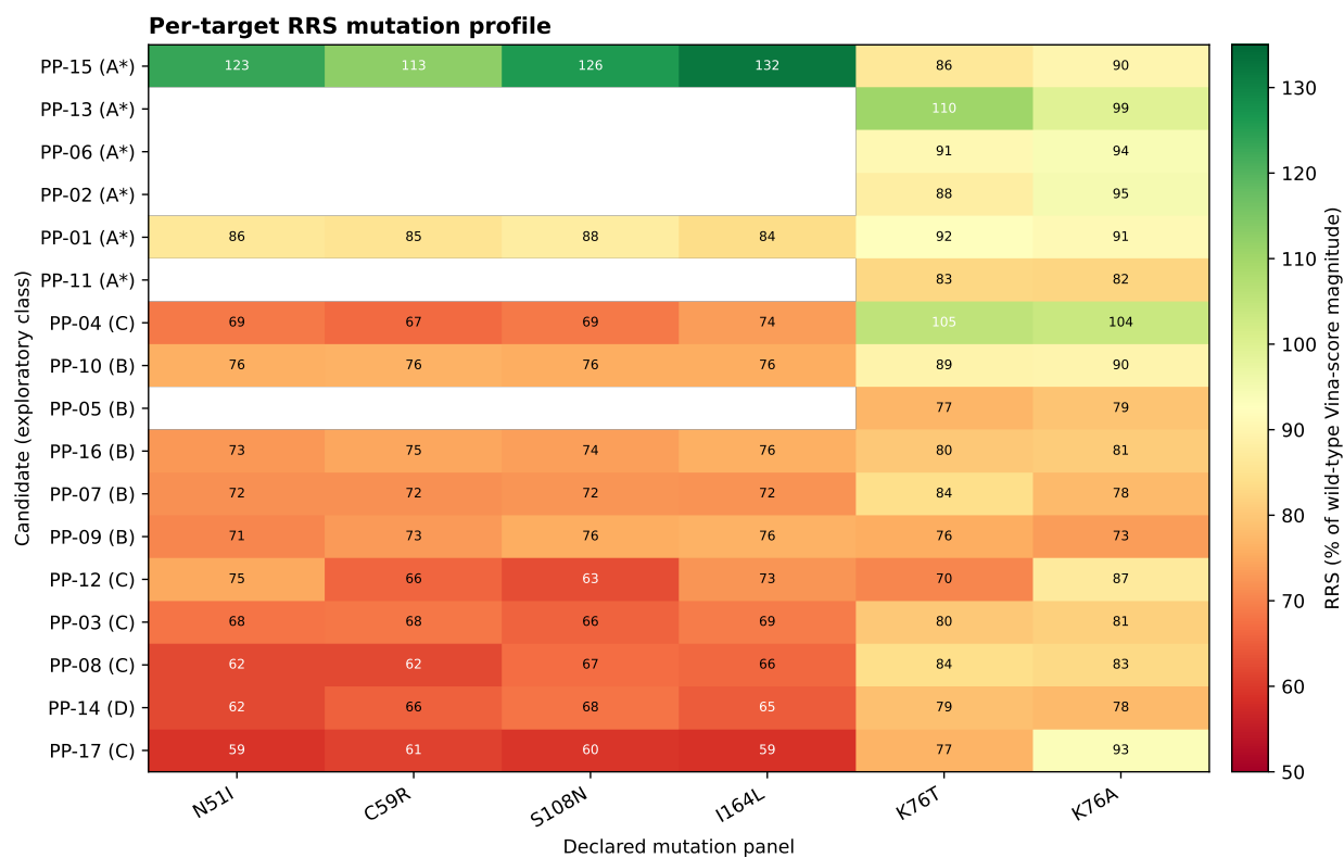
Figure 1: Exploratory per-target RRS mutation profiles for the 17-member source-panel cohort. Values are ratios of Vina-score magnitudes relative to the declared wild-type denominator; blank cells indicate excluded non-binding wild-type targets. The classes are computational operational categories, not biological resistance phenotypes.
