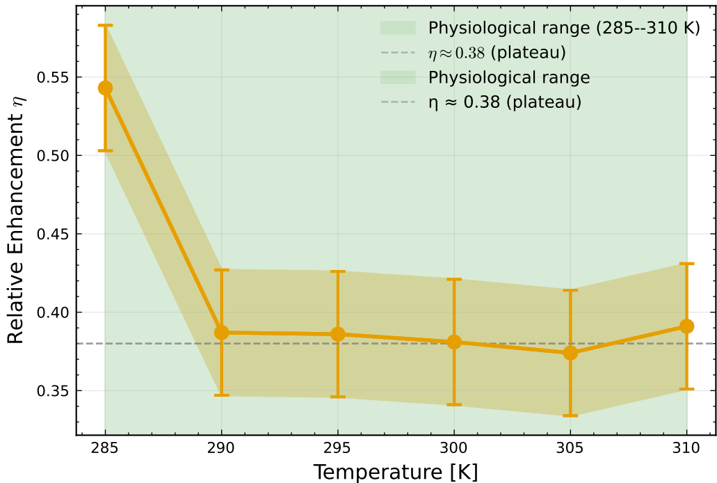
Temperature Dependence of \eta ( L = 7, N = 15 )
