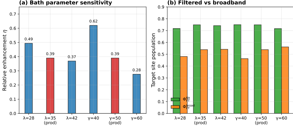
Figure S3: Bath parameter sensitivity ( L = 7 , N = 5 ). (a) Relative enhancement \eta for \lambda_D and \gamma_D variations of \pm 20\% . Red bars indicate the production parameters ( \lambda_D = 35 \text{ cm}^{-1} , \gamma_D = 50 \text{ cm}^{-1} ). (b) Decomposition into filtered and broadband target-site populations. Numerical labels above bars give exact \eta values.
