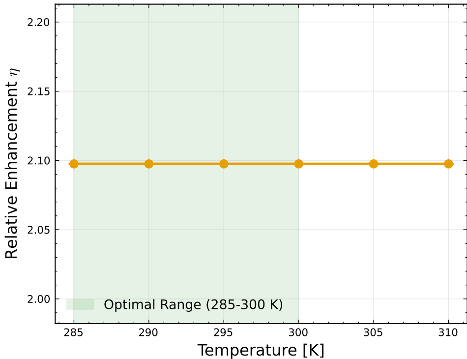
(a) Temperature Dependence
