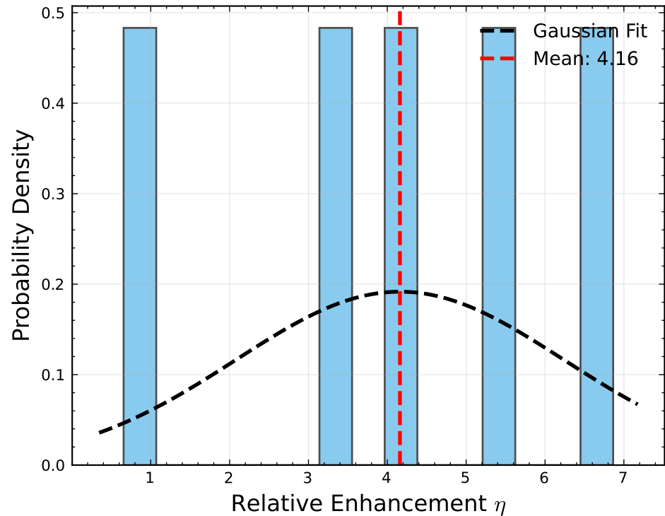
(b) Disorder Robustness ( \sigma = 50 \text{ cm}^{-1} )
