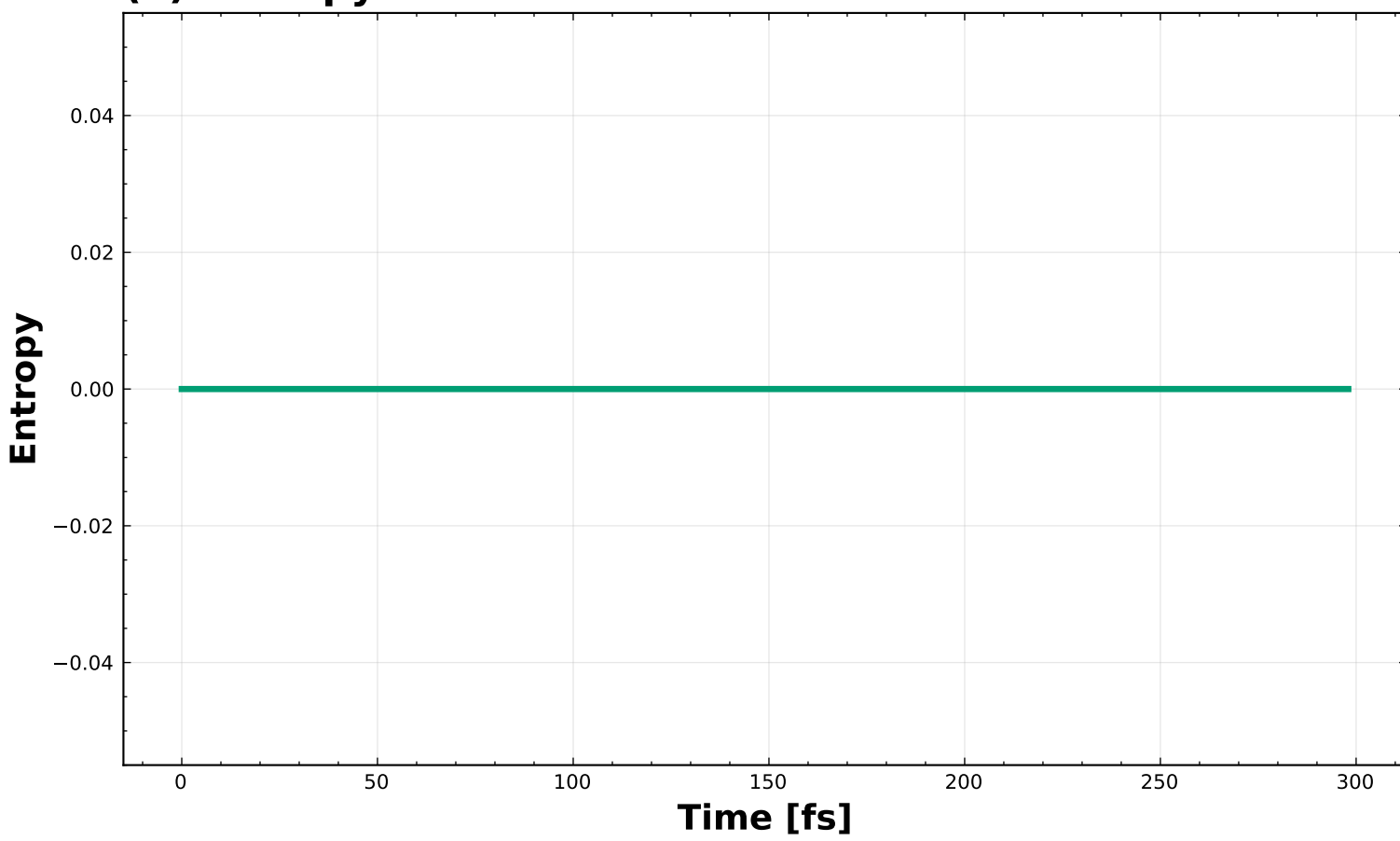
(e) Entropy
