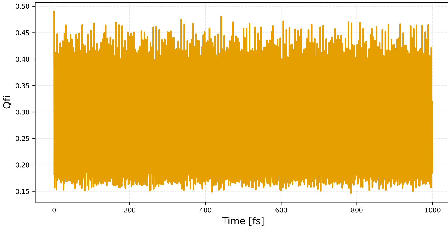
(c) Qfi Evolution
