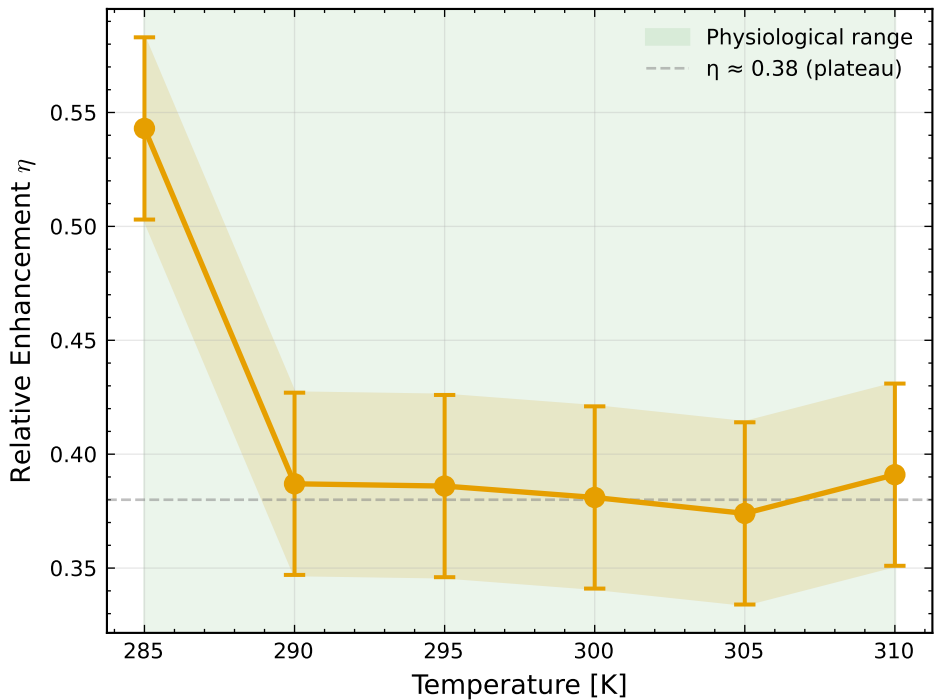
Temperature Dependence of \eta ( L = 7 , N = 15 )
